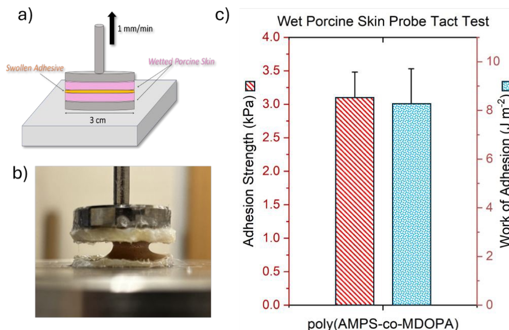
Figure 3. a) Illustration of probe tack test experiments b) photo of poly(AMPS-co-MDOPA) probe tack testing on porcine skin c) poly(AMPS-co-MDOPA) adhesion strength and work of adhesion on porcine skin.
