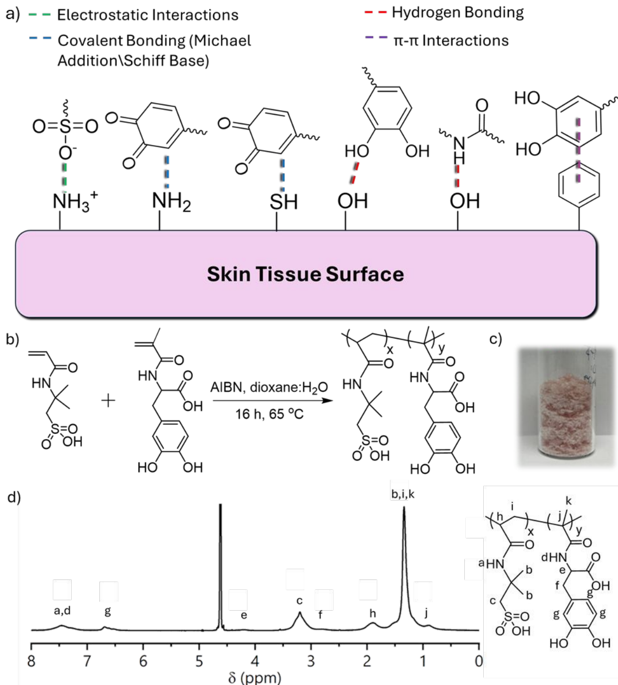
Figure 1. a) Available skin tissue functional groups adhesion mechanisms of poly(AMPS-co-MDOPA) chemical moieties onto skin tissue (concentration of functional groups shown may vary on location) b) Chemical scheme of poly(AMPS-co-MDOPA) synthesis c) A photo of dried poly(AMPS-co-MDOPA) following lyophilization to powder form d) ^1\text{H} NMR spectrum of poly(AMPS-co-MDOPA)
