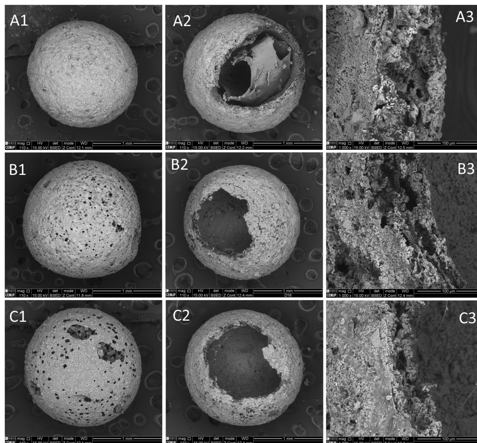
Fig. 7 SEM images of HDS2 at days 1, 16 and 28. Day 1 – whole system (A1); core and shell structure (A2), shell detail (A3). Day 16 – whole system (B1); core and shell structure (B2), shell detail (B3). Day 28 – whole system (C1); core and shell structure (C2), shell detail (C3). Scale bar for pictures A1, A2, B1, B2, C1 and C2 is 1 mm. Scale bar for pictures A3, B3 and C3 is 100 \mu m.
