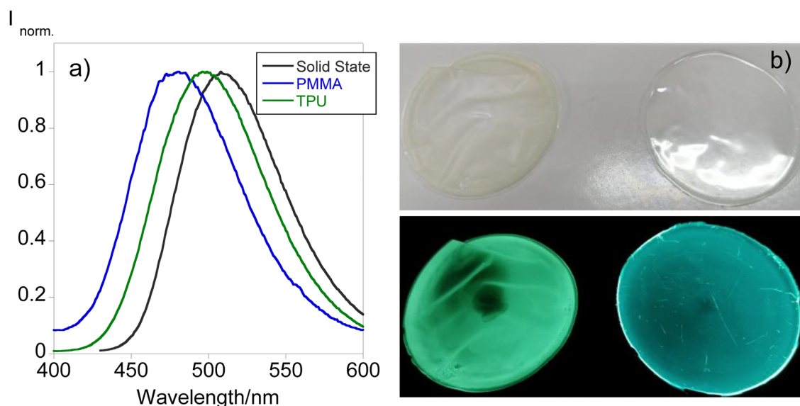
Fig. 5 Comparison between the emission spectra of the different polymer thin films doped with (a) L1 and the (b) images under natural (up) and UV light (down) of TPU (left) and PMMA (right).
