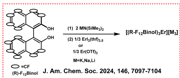
Scheme 40 Chemical structures of the ligands and Ln complexes [(R/S\text{-}F_{12}\text{Binol})_3\text{Er}][M]_3 . 90
