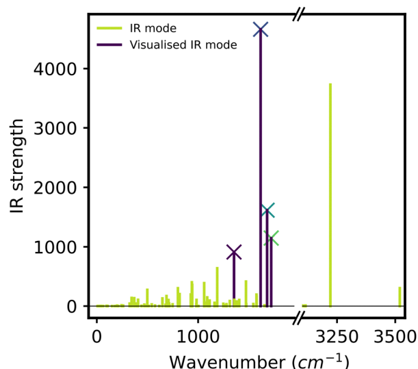
Fig. 9 Spine plot of modes found via density functional theory calculations, shown with vertical lines against their predicted infra-red activity strength. Modes which are visualised and shown in Fig. 12 are shown in purple, with colour-coded X markers at their maximum value, while those not visualised are shown in green.
