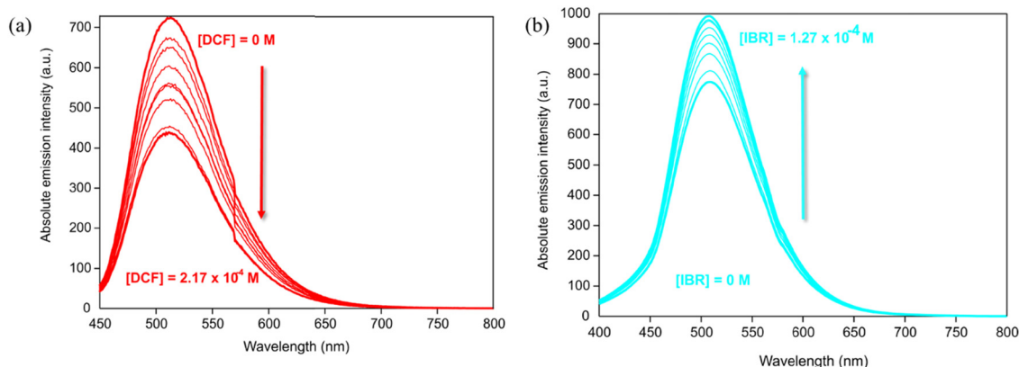
Fig. 4 Emission spectra of Zr_BTDZ ( \lambda_{\text{ex}} = 380 nm) as a function of DCF (a) and IBR (b) concentration in aqueous solution.
