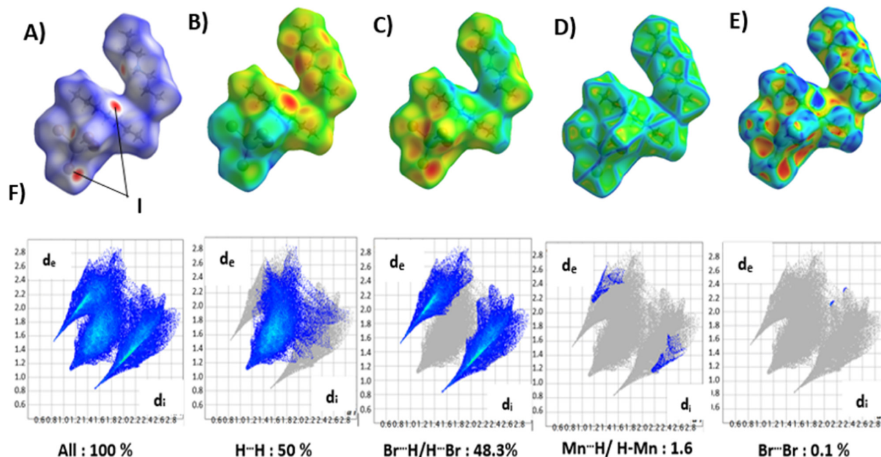
Fig. 2 3D Hirshfeld surfaces mapped over (A) d_{\text{norm}} (close contacts are presented by red spots), (B) d_i , (C) d_e , (D) curvedness, (E) shape index representations (F) 2D fingerprints resolved into all, H...H, Br...H/H...Br, Mn...H/H...Mn and Br...Br contacts, showing the contribution to the total Hirshfeld surface area.
