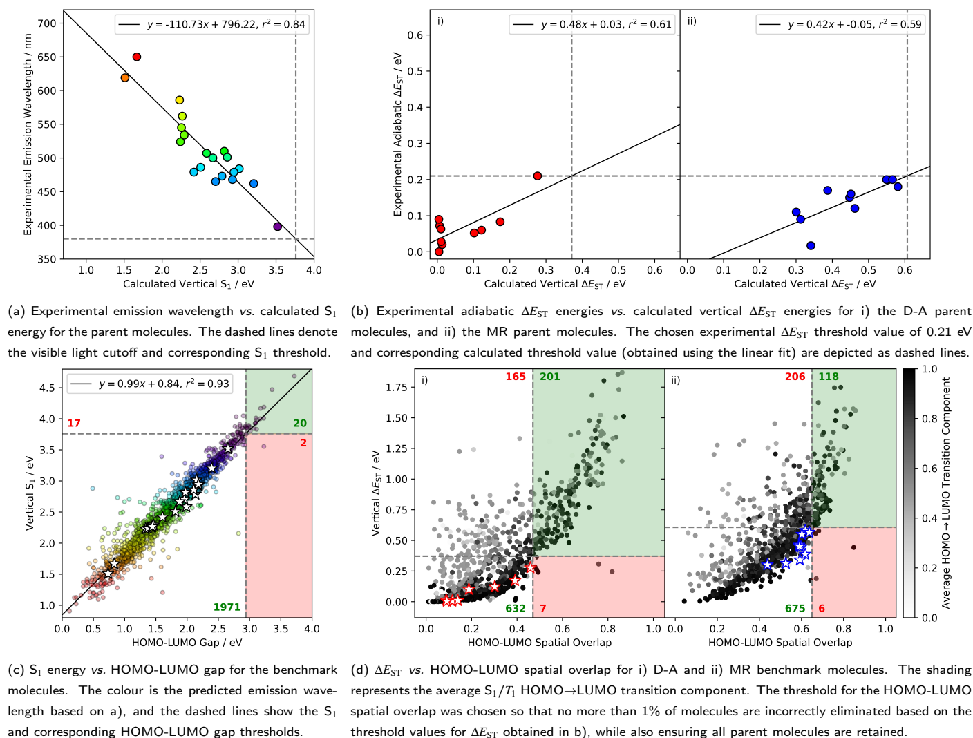
Fig. 3 Benchmarking plots for determining the screening thresholds for HOMO-LUMO gaps and overlaps. The green (red) shaded regions in c) and d) show molecules which are correctly (wrongly) eliminated following the HOMO-LUMO calculation. The corresponding numbers of molecules are written in green (red), as are those which are correctly (needlessly) retained in the unshaded areas. For c) and d) parent molecules are highlighted using the ★ symbol. S_1 , \Delta E_{ST} and HOMO→LUMO transition components were calculated using TDDFT at the B3LYP/6-31G* level on the DFT-optimised geometries, while HOMO-LUMO gaps and overlaps were calculated using PBE and a wavelet basis on the xTB-optimised geometries. Experimental values are from Refs 9,12,70–87 ; the \Delta E_{ST} value for DHPZ-2TRZ is recorded as “nearly zero”, and so was approximated to zero.
