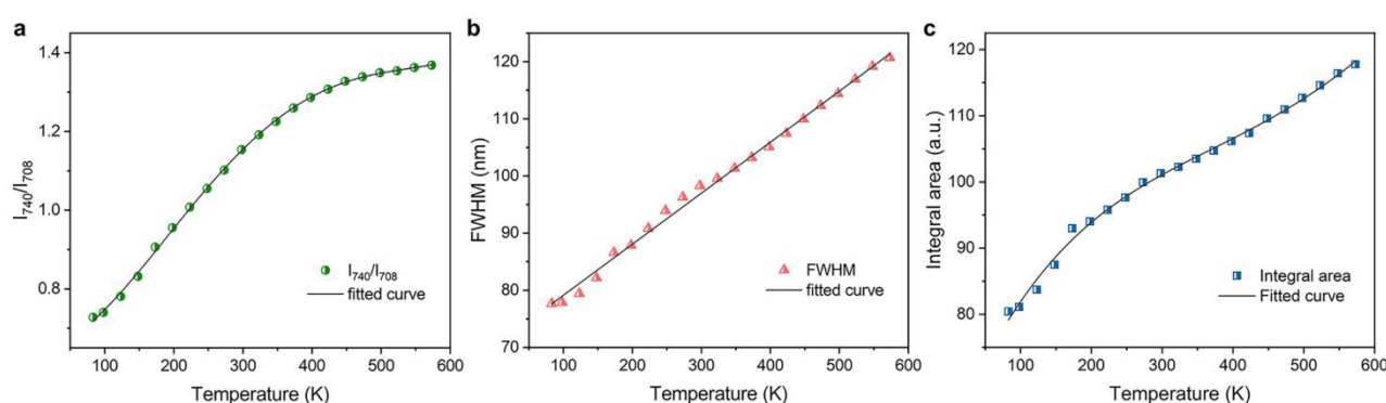
Fig. 6. (a) Peak intensity ratio, (b) FWHM, and (c) integral area of K_2NaGaF_6:Cr^{3+} nanophosphors as function of the temperature.
