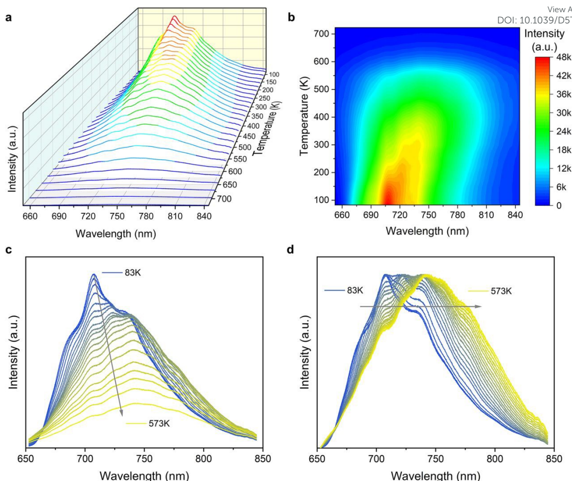
Fig. 4. (a) PL spectra and (b) PL mapping of \text{K}_2\text{NaGaF}_6:\text{Cr}^{3+} nanophosphors as a function of temperature range of 83 K–723 K. (c) Original and (d) normalized PL spectra of \text{K}_2\text{NaGaF}_6:6 \text{ mol\% Cr}^{3+} nanophosphors under the different temperatures.
