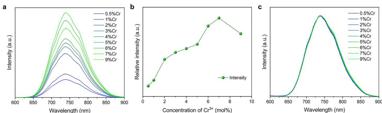
Fig. 1. (a) PL spectra, (b) peak intensity, and (c) normalized emission spectra of \text{K}_2\text{NaGaF}_6 nanophosphors doped with different \text{Cr}^{3+} concentrations.
