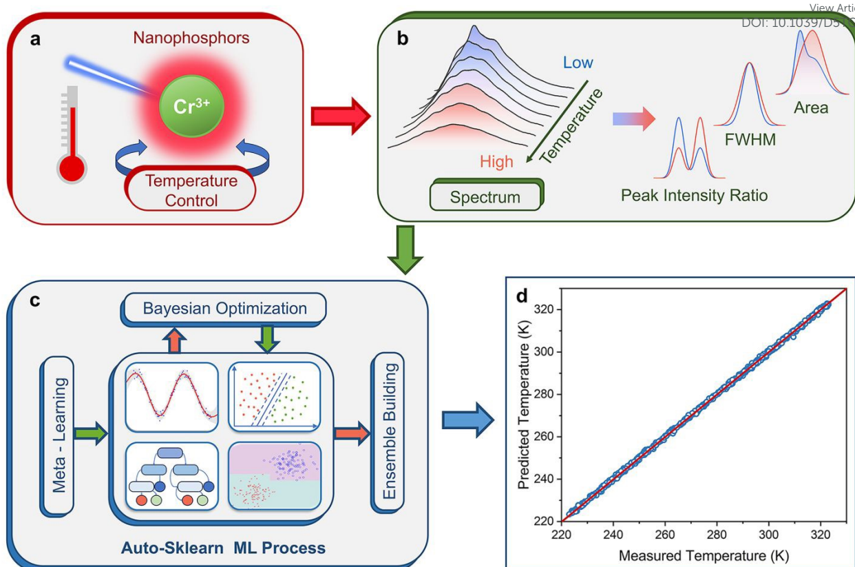
Fig. 7. (a) Schematic diagram of Cr 3+ -doped nanophosphors thermometer. (b) The multi-feature of the spectral data for ML process. (c) The Auto-Sklearn ML process. (d) Predicted vs measured temperature using the ML model.
