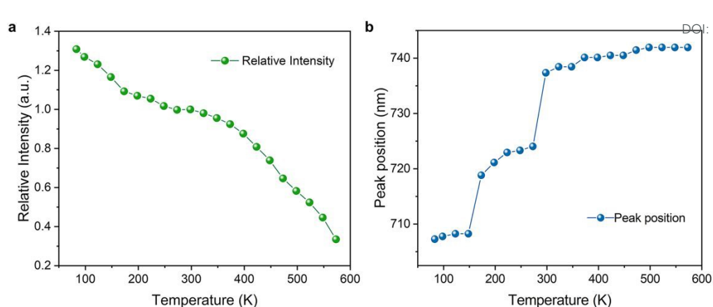
Fig. 5. (a) Relative intensity and (b) maximum peak position of the K_2NaGaF_6:Cr^{3+} nanophosphors as a function of temperature.
