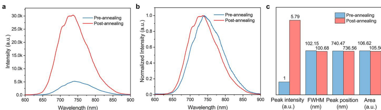
Fig. 2. (a) PL spectrum, (b) normalized PL spectrum, and (c) maximum peak intensity, FWHM, maximum peak position, and integral area of the \text{K}_2\text{NaGaF}_6:6 \text{ mol\% Cr}^{3+} nanophosphors pre- and post-annealing at 873 K temperature.
