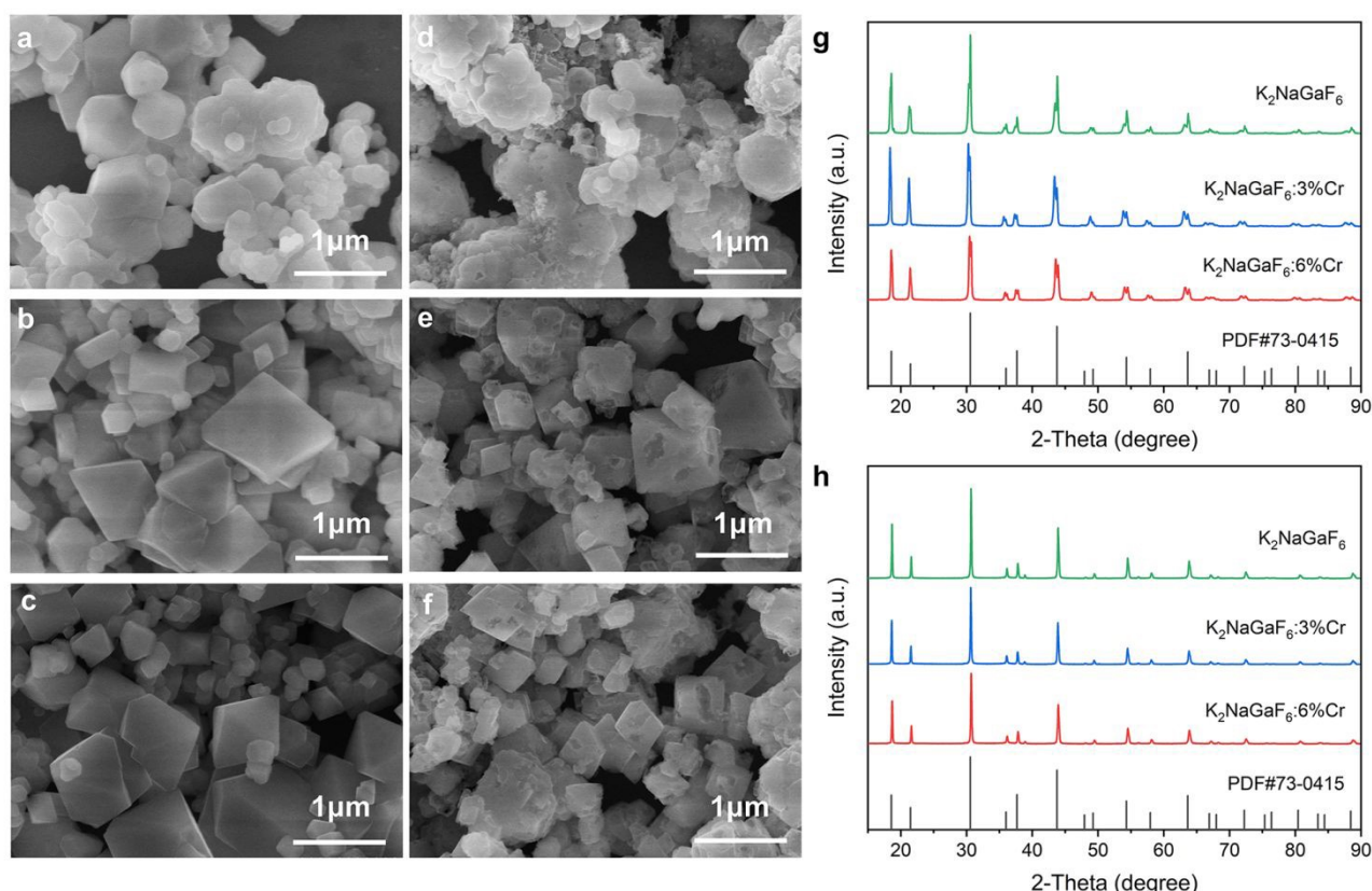
Fig. 3. SEM images of \text{K}_2\text{NaGaF}_6:\text{Cr}^{3+} nanophosphors doped with (a) 0 mol% (b) 3 mol% (c) 6 mol% \text{Cr}^{3+} concentrations before annealing. SEM images of \text{K}_2\text{NaGaF}_6:\text{Cr}^{3+} nanophosphors doped with (d) 0 mol% (e) 3 mol% (f) 6 mol% \text{Cr}^{3+} after annealing. XRD patterns of \text{K}_2\text{NaGaF}_6:\text{Cr}^{3+} nanophosphors doped with different \text{Cr}^{3+} concentrations (g) before annealing and (h) after annealing.
