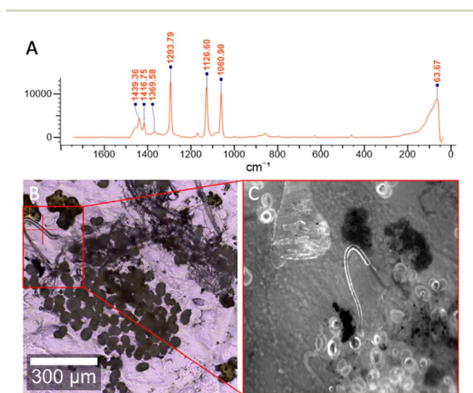
Fig. 2 Identification and labelling of low-density polyethylene microplastic fiber found in a freeze-dried Harp Lake outflow sample. The Raman spectrum in panel (A) corresponds to the fiber marked with a red '+' in panel (B). This spectrum matches low density polyethylene plastic. Panel (C) shows a fluorescent image taken with a fluorescein filter set of this fiber labeled with a 10 pM F-HA-CPN probe solution. Scale bar is 300 microns.
