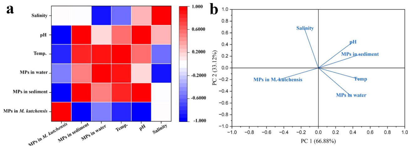
Fig. 6 (a) Pearson's correlation and (b) principal component analysis between microplastic contamination in prawns, sediment, water and environmental matrices (temperature, pH, and salinity).
