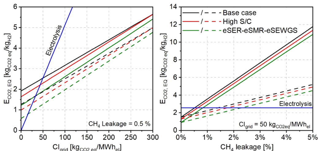
Fig. 10 E_{\text{CO}_2,\text{eq}} for the base case, high steam to carbon, and eSER–eSMR–eSEWGS plants as a function of \text{Cl}_{\text{grid}} (left) and \text{CH}_4 leakage (right). Solid lines refer to GWP20 and dashed lines to GWP100.
