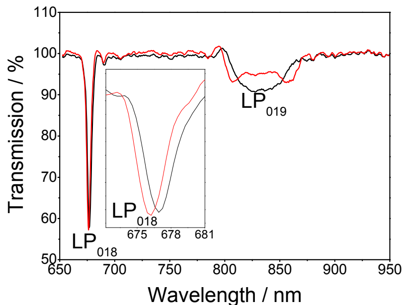
Figure 1. TS of the LPG measured in air: black line, before APTMS deposition, and red line, after APTMS deposition
