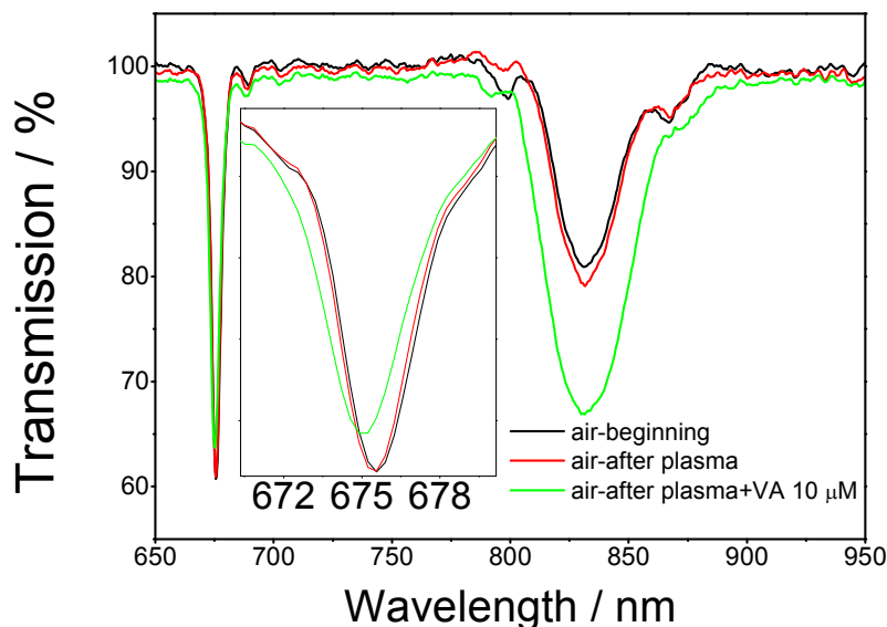
Figure 4. TS of the nano-MIP coated LPG, measured in air before (black line) and after exposure to, porcine plasma (red line) and porcine plasma spiked with 10 \mu\text{M} of VA (green line)
