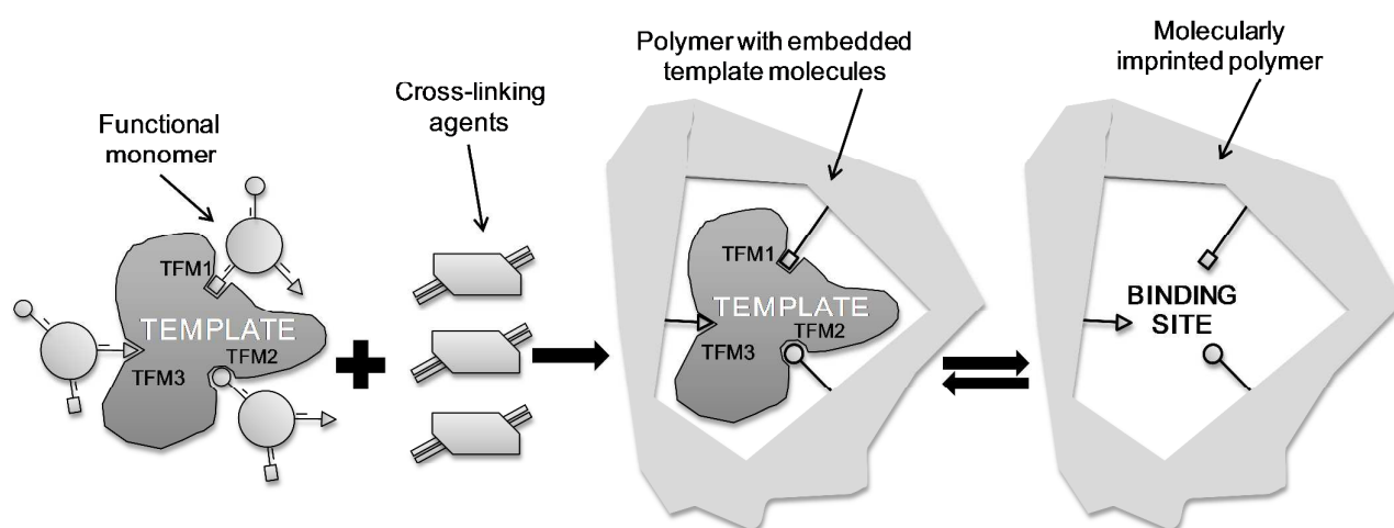
Scheme 1. Schematic illustration of the molecular imprinting procedure 3 .
