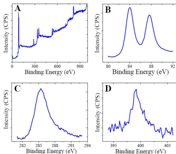
Fig. 4 XPS of CMC-AuNPs: (A) survey spectrum and enlarged XPS spectra for CMC-AuNPs in the (B) Au4f, (C) C1s and (D) N1s regions.
