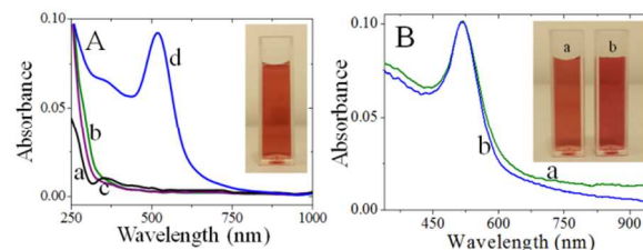
Fig. 1 A) UV-visible spectra of (a) CMC, (b) HAuCl 4 and (c) after the addition of HAuCl 4 to CMC and (d) addition of NaBH 4 to a mixture of HAuCl 4 and CMC. Inset A: Photograph of CMC-AuNPs. B) UV-visible spectra of freshly prepared CMC-AuNPs and after one month old CMC-AuNPs. Inset B: Photograph of freshly prepared and one month old CMC-AuNPs.
