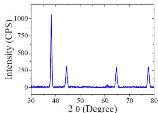
Fig. 3 X-Ray diffraction pattern of as-prepared CMC-AuNPs.
