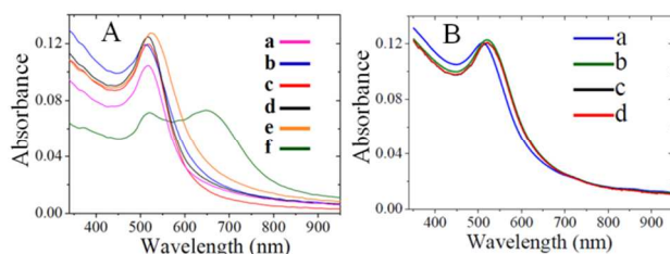
Fig. 8 (A) Absorption spectra obtained after the addition of 1.7 \times 10^{-13} M T7 viruses into different AuNPs solution under optimized conditions: (a) citrate-AuNPs, (b) CTAB-AuNPs, (c) PAA-AuNPs, (d) PL-AuNPs, (e) glucose-AuNPs and (f) CMC-AuNPs. (B) Absorption spectra obtained for (a) CMC-AuNPs, (b) CMC-AuNPs in PBS medium, (c) after addition of 1 \times 10^{-6} M bovine serum albumin (BSA) protein into CMC-AuNPs solution and (d) the solution "c" after 1 hr, under optimized conditions.
