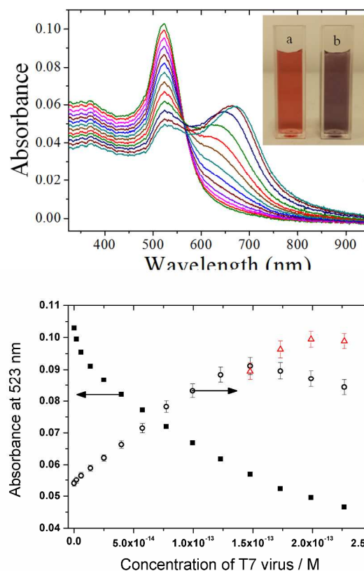
Fig. 7 (A) UV-visible spectra of CMC-AuNPs in different concentrations of T7 virus: 0 M, 2.0 \times 10^{-15} M, 5.9 \times 10^{-15} M, 1.4 \times 10^{-14} M, 2.5 \times 10^{-14} M, 4.0 \times 10^{-14} M, 5.7 \times 10^{-14} M, 7.7 \times 10^{-14} M, 9.9 \times 10^{-14} M, 1.2 \times 10^{-13} M, 1.5 \times 10^{-13} M, 1.7 \times 10^{-13} M, 2.0 \times 10^{-13} M, and 2.3 \times 10^{-13} M. Inset: photographs of CMC-AuNPs before (a) and after (b) the addition of T7 viral phages. (B) Calibration curve for CMC-AuNPs in 2.0 \times 10^{-15} – 2.3 \times 10^{-13} M concentrations of T7 virus (for details see text).
