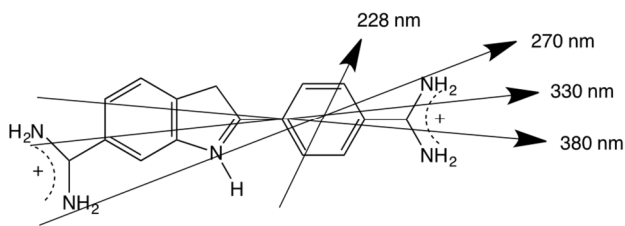
Figure 7. 4',6-Diamidino-2-phenylindole illustrating approximate transition polarizations consistent with this work and the PVA data of reference. 26
