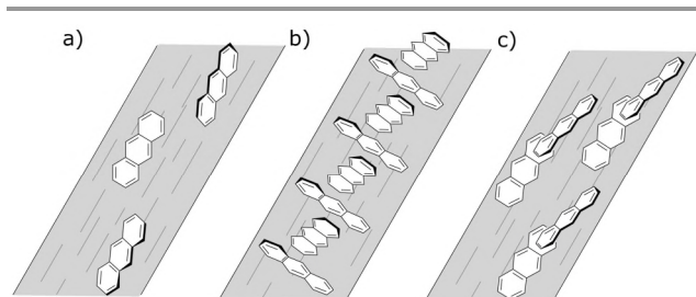
Figure 11. The three proposed orientations of anthracene on PE OX films, a) uniaxially oriented single molecules, b) extended cross-hatched structure and c) skewed dimers.
