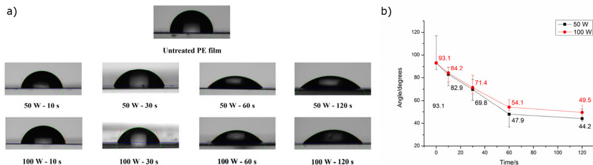
Figure 2. a) Water drops on polyethylene films treated at the indicated power levels for the indicated times. b) The contact angle of PE films placed in the plasma asher at different power levels as a function of time.
