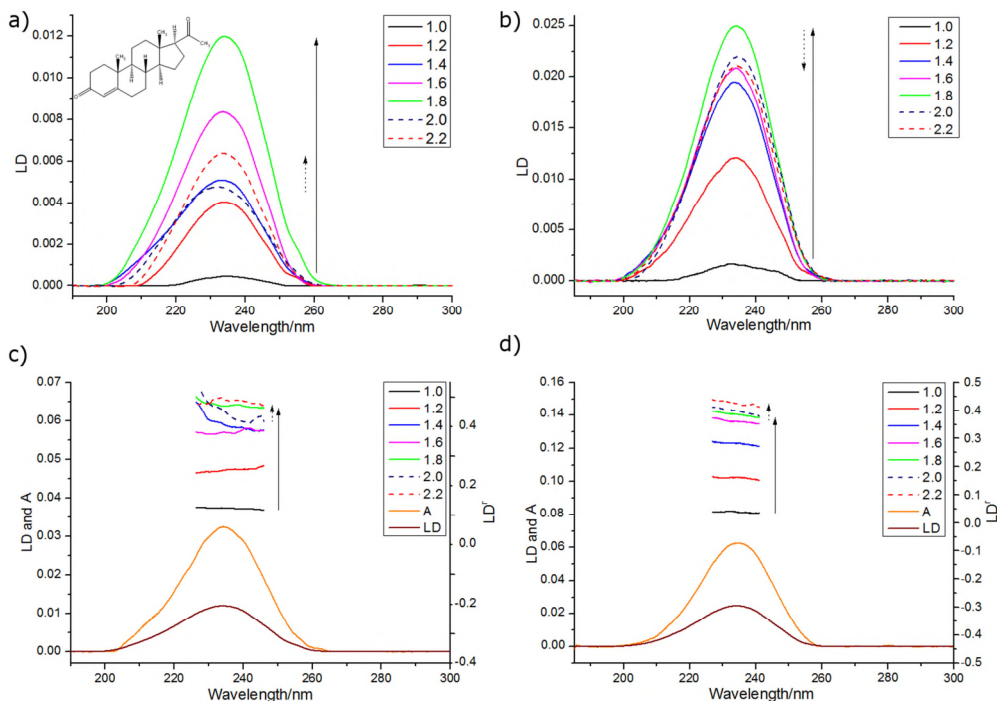
Figure 4. Spectra of progesterone (deposited from 0.65 mg/mL in chloroform for PE and methanol for PE OX and left to dry). LD on a) PE, and b) PE OX prestretched by factors ranging from 1 to 2.2. c) and d) LD f for data from (a) and (b) respectively overlaid with absorbance and LD spectra for \times 1.8 stretch.
