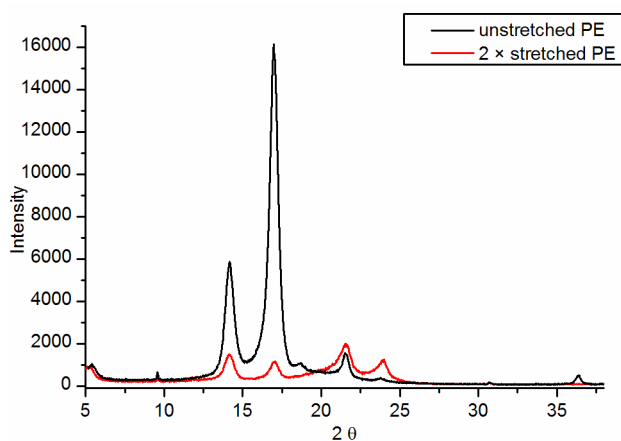
Figure 3. X-ray diffraction patterns of un-stretched and 2× stretched PE films.
