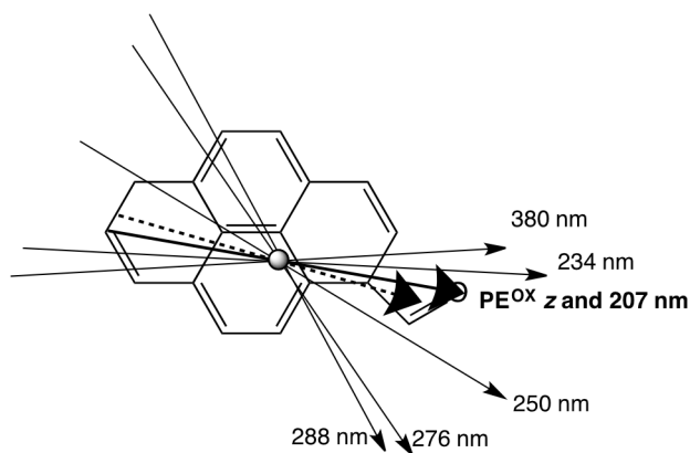
Figure 9. Polarizations of PyCO transitions assuming the orientation direction of PE OX is as indicated by the thick solid line (the longest molecular axis with O lying flat on the film). The thick dashed line is then the orientation axis on PE.
