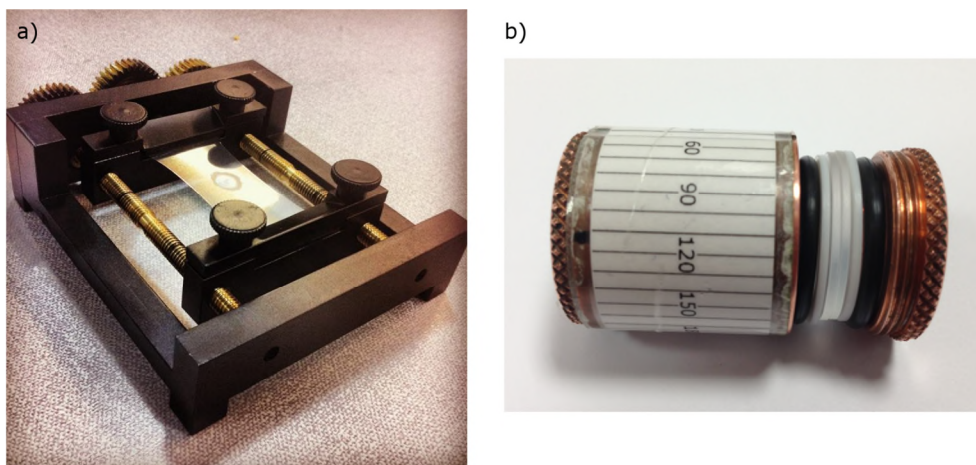
Figure 1. a) Mechanical film stretcher designed and built at the University of Warwick. b) Cylindrical film holder (originally designed for oriented circular dichroism measurements) 19 where film is held between two quartz plates (1 mm thick) themselves sandwiched between Teflon rings and O-rings.
