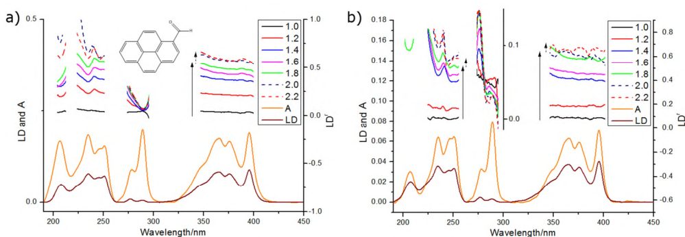
Figure 8. LD f spectra of pyrenecarboxaldehyde (deposited from 0.4 mg/mL in methanol and left to dry) on films prestretched by factors ranging from 1 to 2.2 × overlaid with absorbance and LD spectra for ×1.8 stretch. (a) PE and (b) PE OX .
