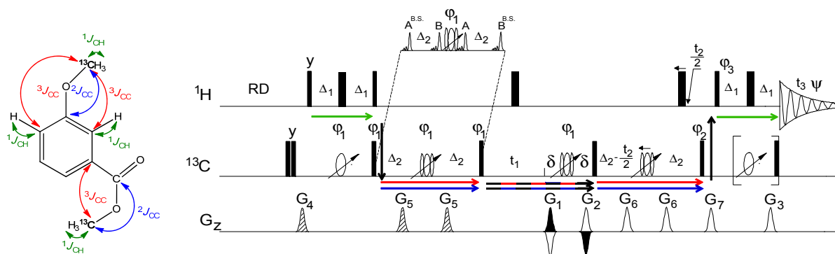
Fig. 1. The pulse sequence of the 3D IPAP INEPT-INADEQUATE-HSQC and its polarisation transfer pathways utilising various coupling constants. The details of the pulse sequence are given in the Supplementary Information.
