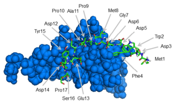
Figure 1 Structure of CXCL8 (blue) in complex with the receptor derived peptide H 2 N-MWDFDDGMPPADEDYSP-COOH (green stick model) used in this work.
