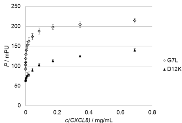
Figure 3 Sample graph for binding experiments. Binding isotherms of the peptide with the highest (D12K, black triangles) and lowest (G7L, white diamonds) K_d value are shown.
