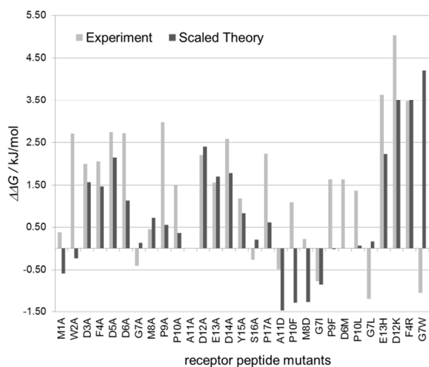
Figure 4 Comparison of theoretical and experimental data (a) When divided by a factor of three theoretical values (dark grey) correspond reasonably well with experimental values (light grey) for binding energy differences.
