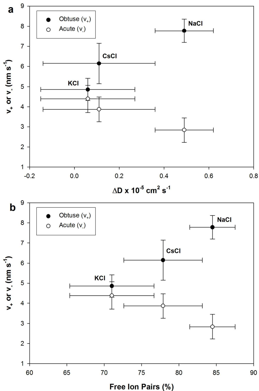
Figure 4. Obtuse ( v_+ ) and acute ( v_- ) step propagation velocities of the calcite{1 0 -1 4} surface, obtained from in situ AFM experiments at IS = 0.02 in NaCl, CsCl and KCl salts, as a function of (a) difference in the diffusion coefficients of ionic salt constituents ( \Delta D ) and (b) concentration of free ions in the simulated NaCl, CsCl and KCl solutions (low IS, 0.06 mol kg -1 )
