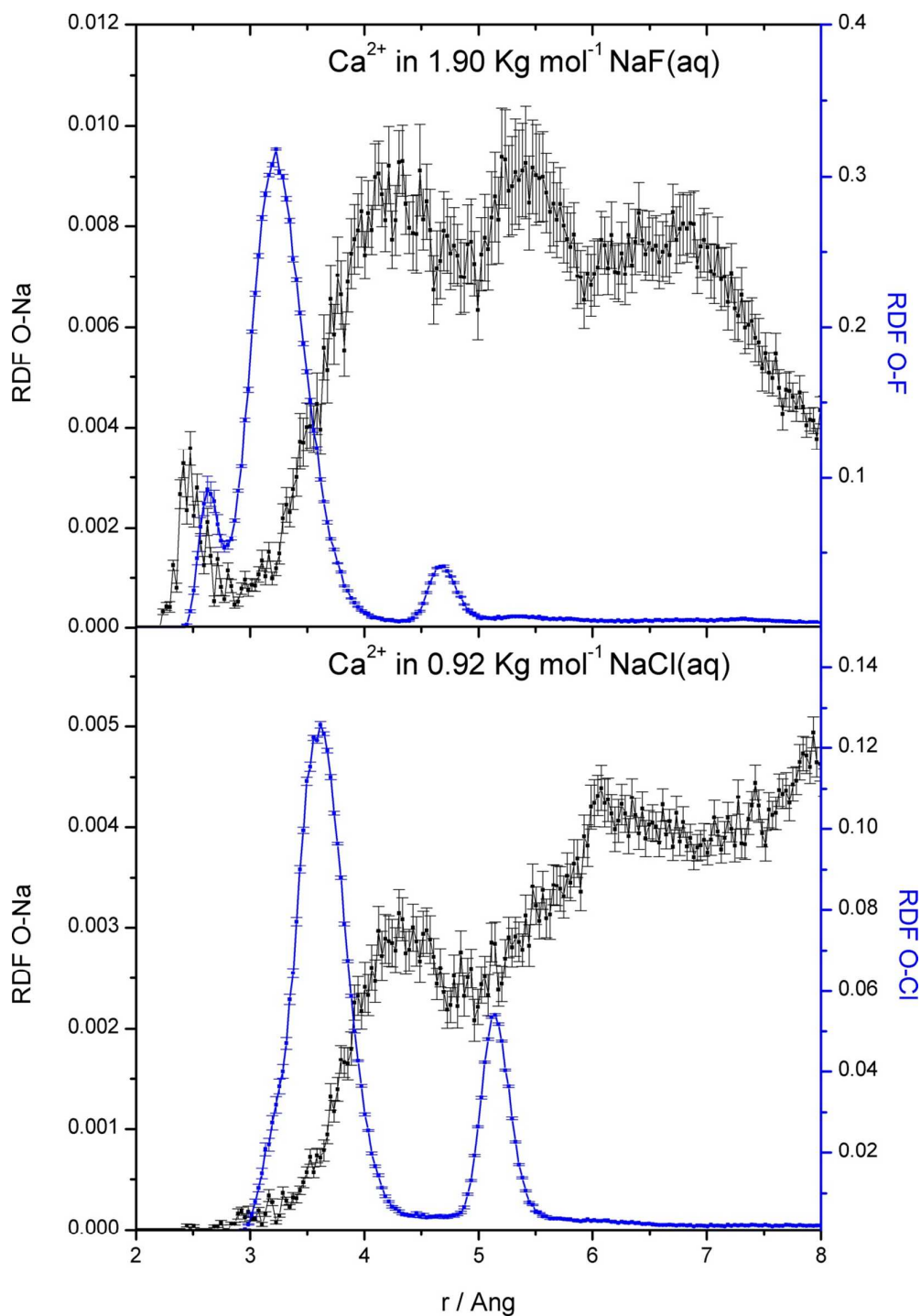
Figure 12. Oxygen-sodium (black line) and oxygen-halide (blue line) radial distribution functions for the water molecules that are part of the first hydration shell of the calcium ion as obtained from the simulations of \text{Ca}^{2+} in the 1.90 mol kg -1 NaCl aqueous solution and 0.92 mol kg -1 NaF aqueous solution.
