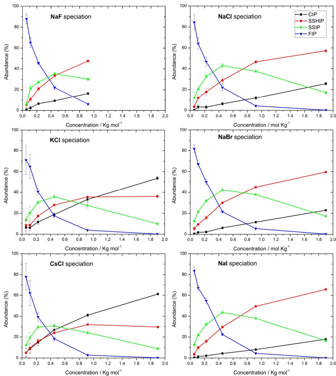
Figure 3. Speciation of alkali halide ion pairs as a function of concentration. The standard errors of the number of percentage of contact ion pairs (CIP), solvent-shared ion pairs (SSHIP), solvent-separated ion pairs (SSIP) and free ion pairs (FIP) have been computed from the variation of 10 block averages within each trajectory.
