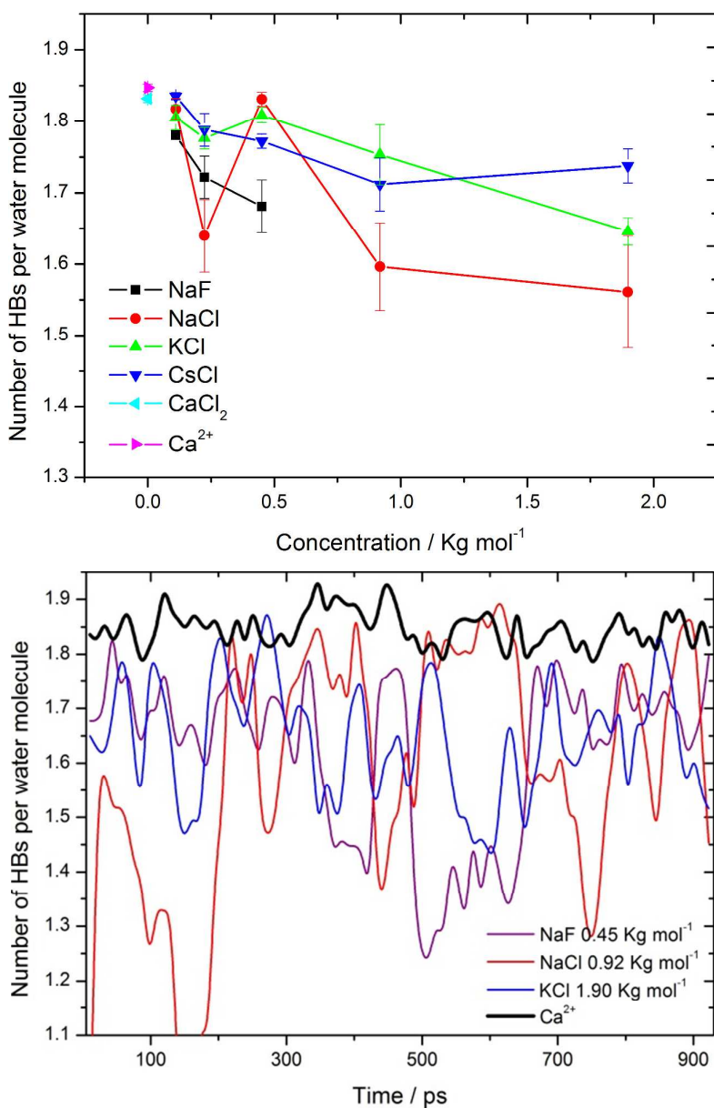
Figure 11. (a) Average number of hydrogen-bonds (HBs) per water molecule for the water molecules that are part of the first coordination shell of \text{Ca}^{2+} as obtained from the molecular dynamics simulations of one calcium ion in bulk water and in aqueous alkali halide solutions at different concentrations. The standard error of the number of HBs has been computed from the variation of 10 block averages within each trajectory. (b) Hydrogen bond fluctuations for the water molecules of the hydration shell of the calcium ion.
