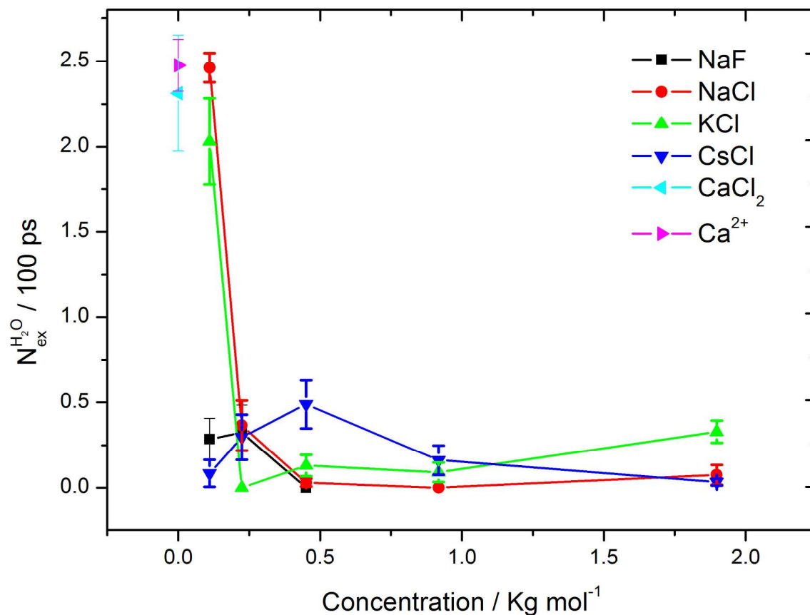
Figure 9. Number of accounted water exchange events ( N_{ex}^{H_2O} ) in the first hydration shell of calcium, with a duration of more than 0.5 ps, obtained from the MD simulations of the calcium ion in water in aqueous alkali halide solutions at different concentrations. The first hydration shell is defined by the coordination limit r(\text{Ca-O}) = 3.4 \text{ \AA} . The values of N_{ex} are normalized to 100 ps and the hydration number of the calcium ion. The standard errors of N_{ex}^{H_2O} have been computed from the variation of 10 block averages within each trajectory.
