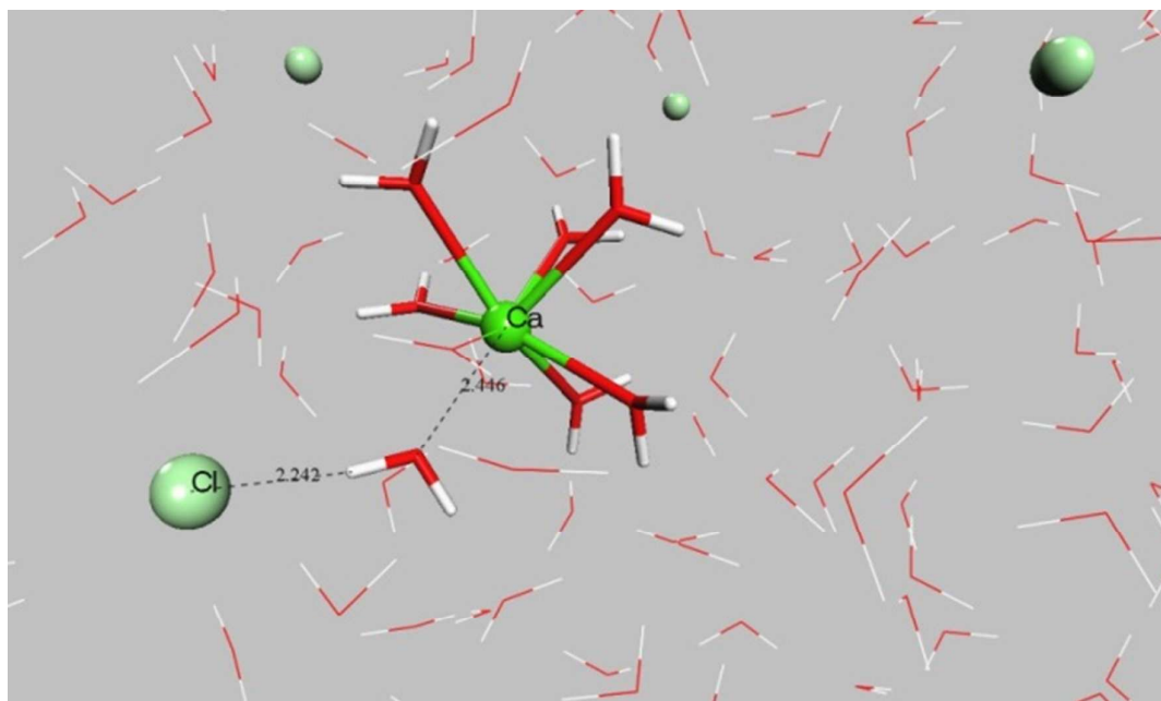
Figure 10. Snapshot of the MD simulation of \text{Ca}^{2+} in \text{KCl} 1.90 \text{ mol Kg}^{-1} solution (last 100 ps).
