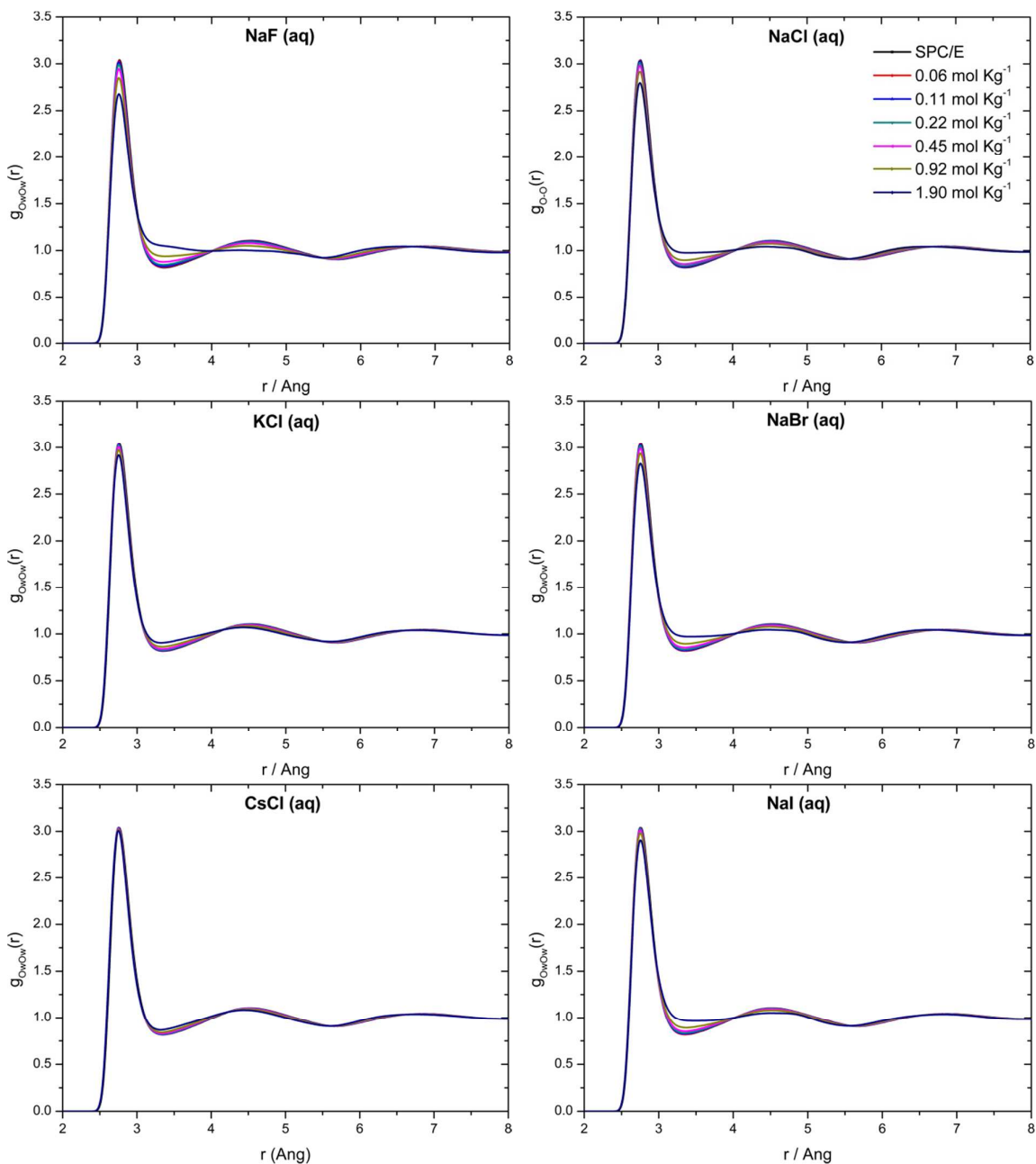
Figure 2. Oxygen-oxygen radial distribution functions in pure SPC/E water and aqueous alkali halide solutions at different concentrations.
