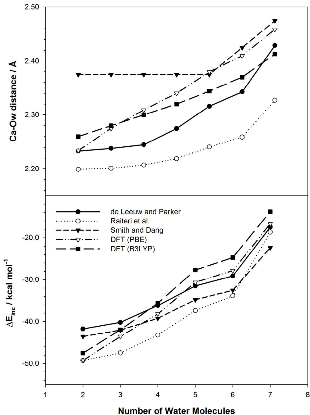
Figure 1. Average \text{Ca}^{2+}\text{-O}_w distance (above) and successive water binding energy of calcium (below) of \text{Ca}(\text{H}_2\text{O})_n^{2+} clusters computed using the Buckingham \text{Ca}^{2+}\text{-O}_w potential parameterized by de Leeuw and Parker, 37 the Lennard-Jones \text{Ca}^{2+}\text{-O}_w potentials parameterized by Dang and Smith, 40 and the Lennard-Jones \text{Ca}^{2+}\text{-O}_w potential parameterized
