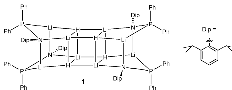
Chart 1 the phosphinoamide stabilized LiH complex 1
