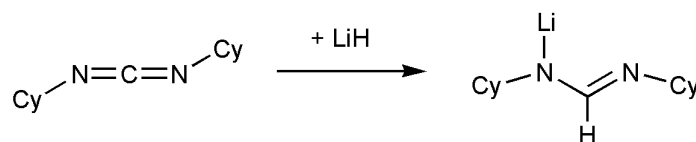
Scheme 1 hydrolithiation of DCC
