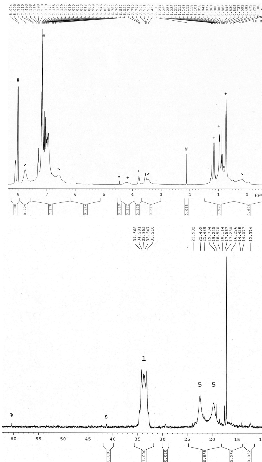
Fig 2. ^1\text{H} NMR (400.17 MHz) spectrum (top) and ^{31}\text{P}\{^1\text{H}\} NMR (161.98 MHz) spectrum (bottom) of the in-situ reaction of [(LLi) 4 (LiH) 4 ] 1 with PhN=NPh at room temperature after ca. 16 h in deuterated benzene recorded at 303 K showing partial conversion to [{(LN(Ph)N(Ph)Li) 2 }] 5 . ^1\text{H} : #: PhN=NPh resonances; *: H 2 ; +: characteristic resonances of [(LLi) 4 (LiH) 4 ] 1 ; >: selected
