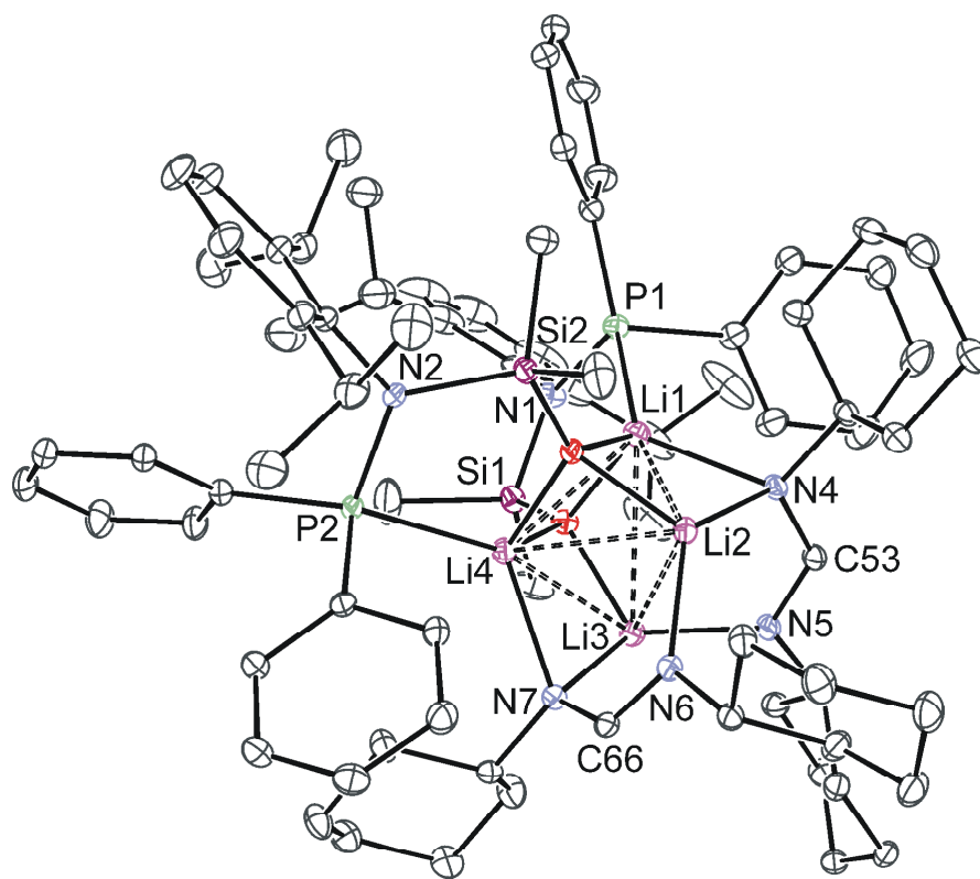
Fig. 1 Molecular structure of compound 3 ·3 C 6 H 6 (30% probability thermal ellipsoids). Hydrogen atoms and solvent molecules have been omitted for clarity. Selected bond lengths (Å) and angles (°): P(1)-N(1) 1.7160(15), P(2)-N(2) 1.7148(13), P(1)-Li(1) 2.651(3), P(2)-Li(4) 2.624(3), Si(1)-O(1), 1.6005(11), Si(2)-O(2) 1.6004(11), Si(1)-N(1) 1.7807(14), Si(2)-N(2) 1.7767(13), O(1)-Li(3) 1.907(3), O(1)-Li(1) 1.921(3), O(1)-Li(4) 1.993(3), Li(1)-O(2) 1.934(3), Li(1)-N(4) 2.132(3), O(2)-Li(2) 1.896(3), O(2)-Li(4) 1.921(3), Li(2)-N(6) 1.938(3), Li(2)-N(4) 2.041(3), Li(3)-N(5) 1.952(3), Li(3)-N(7) 2.070(3), Li(4)-N(7) 2.135(3), N(4)-C(53) 1.3384(19), N(5)-C(53) 1.303(2), N(6)-C(66) 1.3048(19), N(7)-C(66) 1.338(2); P(1)-N(1)-Si(1) 116.46(8), P(2)-N(2)-Si(2) 117.49(7), Li(3)-O(1)-Li(4) 79.76(12), Li(1)-O(1)-Li(4) 81.96(11), Li(3)-O(1)-Li(1) 96.93(12), N(5)-C(53)-N(4) 125.10(13), N(6)-C(66)-N(7) 125.30(14).
