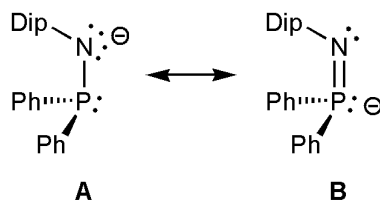
Chart 2 phosphinoamide and iminophosphide mesomeric forms of L^-
