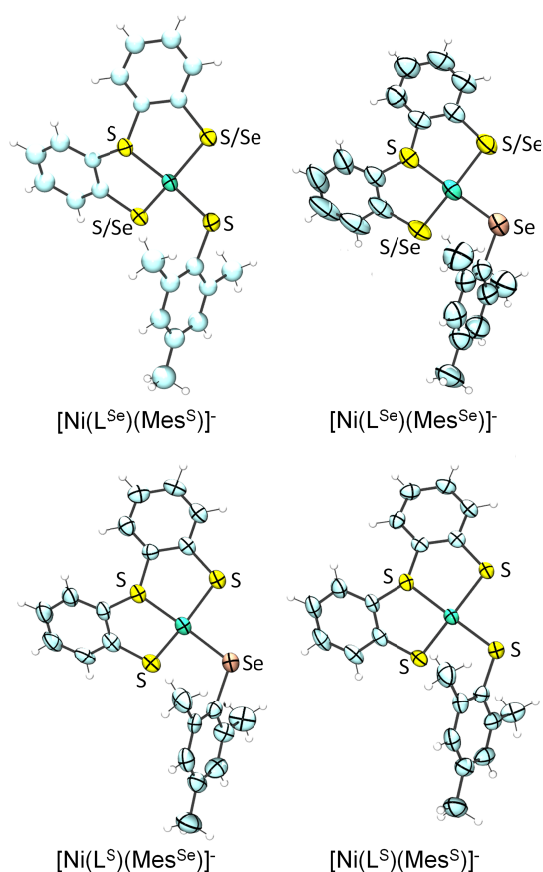
Figure 3. X-ray single crystal structures of complexes ( n -Bu 4 N)[Ni(L E )(Mes E' )] showing 50% probability ellipsoids (counterion not shown; the asymmetric units of [Ni(L Se )(Mes S )] - , [Ni(L S )(Mes Se )] - and [Ni(L S )(Mes S )] - contain two independent anions; images created using Ortep 3 for Windows 15 ).
