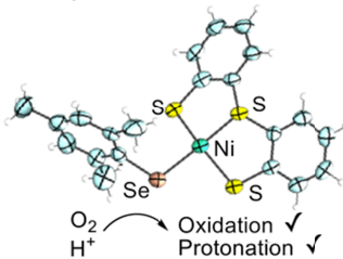
Synthetic Ni site model
