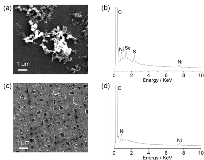
Figure 5. SEM images and EDX spectra of a (a and b) Ni particle modified glassy carbon electrode prepared from the electro-deposition of (n\text{-Bu}_4\text{N})[\text{Ni}(\text{L}^{\text{Se}})(\text{Mes}^{\text{S}})] (1 mM) and (c and d) Ni film on a glassy carbon electrode prepared from the electrodeposition of \text{Ni}(\text{NO}_3)_2 \cdot 6\text{H}_2\text{O} (1 mM). The deposits were formed with the compounds at an applied potential of -1.33 \text{ V vs. NHE} for 0.5 h in acetonitrile (0.1 M n\text{-Bu}_4\text{NBF}_4 ) with \text{Et}_3\text{NHCl} (10 mM).
