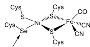
[NiFeSe] hydrogenase active site
