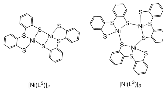
Figure 2. Chemical structure of [Ni(L S ) n ] in the dimeric ( n = 2 ) 12l and trimeric ( n = 3 ) 12l form.
