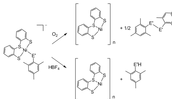
Scheme 2. Reactivity of [Ni(L S )(Mes Se )] (E' = Se) and [Ni(L S )(Mes S )] (E' = S) with O 2 and HBF 4 .
