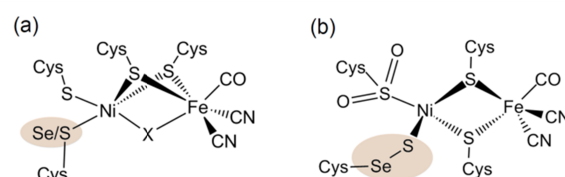
Figure 1. (a) Molecular structure of the [NiFe(Se)] hydrogenase active site. The highlighted atom is S in [NiFe] hydrogenases and Se in [NiFeSe] hydrogenases. A hydride or oxo-group can serve as the bridging moiety X (the latter was only observed in oxidised [NiFe] hydrogenases) and an active reduced state does not contain a bridging ligand X. (b) Composition of a structural conformer in the oxidised [NiFeSe] hydrogenase from Desulfovibrio vulgaris Hildenborough. 9f, 9g, 10
