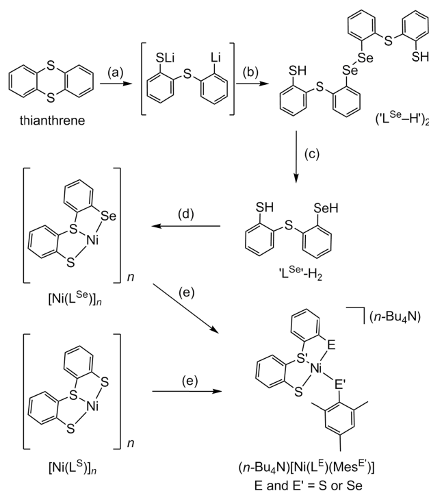
Scheme 1. Synthetic pathway to models of the Ni-site in [NiFe(Se)] hydrogenases: (a) Li, 4,4'-di- tert -butylbiphenyl, tetrahydrofuran, -90 °C. (b), (i) Se, -90 °C to -50 °C; (ii) H 3 O + . (c), (i) NaBH 4 ; (ii) H 3 O + . (d) Ni(OCOCH 3 ) 2 ·4H 2 O, tetrahydrofuran/methanol, reflux. (e) NaMes E' (E' = S or Se), n -Bu 4 NOH, tetrahydrofuran/methanol.
