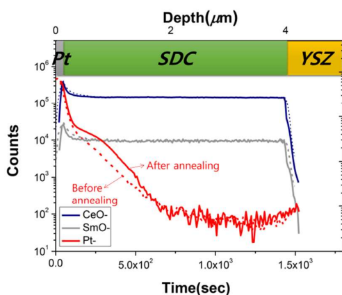
Figure 3. Depth profile of Pt (red), Ce (blue triangle), and Sm (gray), obtained by SIMS analysis. Substantial amounts of elemental Pt are detected even deeper than 1 \mu\text{m} from the top surface. The effect of annealing at 700 °C (2 h, air) on the depth profile of each element is shown (dotted line: before annealing, solid line: after annealing).
