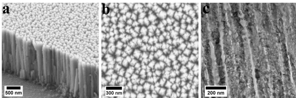
Figure 1. SEM and TEM micrographs of the porous columnar SDC films prepared by PLD in 100 mTorr O_2 at 650 °C prior to metal deposition. (a) SEM image (cross-sectional view after tilting the sample by 45 °). (b) SEM image (top view). (c) TEM image (cross-sectional view), indicating vertical pore-channels with a width of less than 20 nm.
