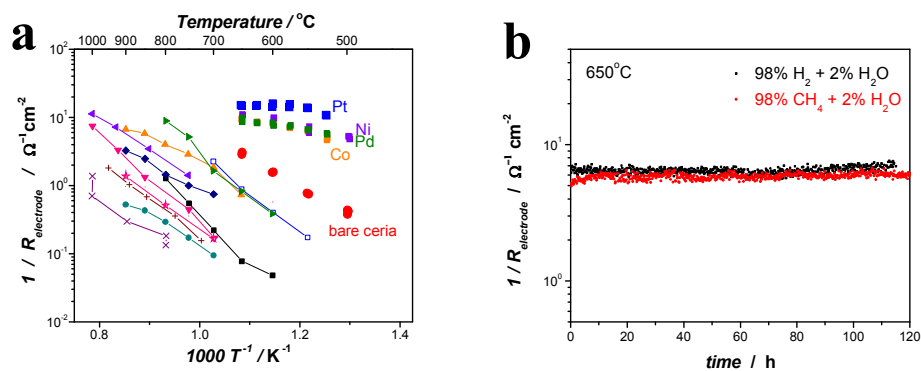
Figure 6. (a) Arrhenius plot of electrode activity (normalized) for the metal-nanoparticle-decorated SDC thin film in this study. For comparison, the reported electrode activity (normalized) values for typical anodes are also inserted. Reference [28] (■) = slurry-coated Ni, (□) = slurry-coated Ni/Fe; reference [29] (▶) = spin-coated Ni/SDC; reference [15] (▲) = Pd impregnated Ni/GDC; reference [30] (▼) = sprayed GDC, (◀) = Ni impregnated GDC; reference [31] (●) = slurry-coated Ni, (◆) = GDC impregnated Ni; reference [32] (☆ half-filled) = slurry-coated GDC; reference [33] (+) = slurry-coated Ni/YSZ; reference [34] (×) = slurry-coated Ni/YSZ. (b) Long term stability of the Pt-nanoparticle-decorated SDC thin film for both H 2 and CH 4 gases, measured at 650 °C, p_{\text{H}_2} = 0.98 atm, and p_{\text{H}_2\text{O}} = 0.02 atm.
