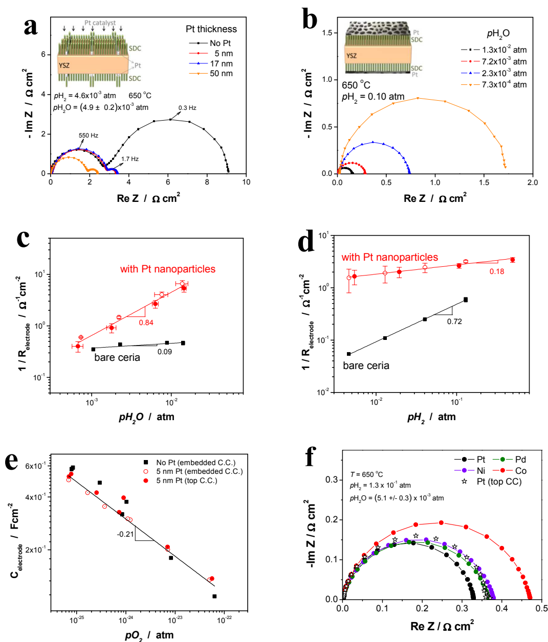
Figure 5. (a) Typical impedance spectra obtained from SDC|patterned Pt|YSZ(100)|patterned Pt|SDC symmetric cells with/without Pt catalysts. The electrode impedance dramatically decreases after depositing a Pt layer onto the SDC films, while it remain nearly identical regardless of the total amount of Pt deposited by sputtering between 5 nm and 50 nm. (b) Typical impedance spectra obtained from a sputtered Pt|SDC|YSZ(100)|SDC|sputtered Pt symmetric cell as a function of p_{H_2O} . Elimination of electronic current constriction effects eliminates the high frequency arc evident in (a). (c) Double-logarithmic plot of the electrode activity (normalized) vs. p_{H_2O} measured at T = 650\text{ }^\circ\text{C} and p_{H_2} = 0.05 - 0.10\text{ atm} . (d) Double-logarithmic plot of the electrode activity (normalized) vs. p_{H_2} measured at T = 650\text{ }^\circ\text{C} and p_{H_2O} = 0.005\text{ atm} . The electrochemical reaction activities of the two types of cells (embedded current collector and top current collector) were indistinguishable. The errors were determined by six different cells (two embedded current collectors and four top current collectors). (e) Double-logarithmic plot of the electrode capacitance (normalized) vs. p_{O_2} measured at T = 650\text{ }^\circ\text{C} . (f) Comparison of impedance spectra obtained from SDC|patterned Pt|YSZ(100)|patterned Pt|SDC symmetric cells with various catalysts (electronic constriction arc removed).
