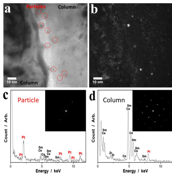
Figure 4. Bright field (a) and dark field (b) TEM images of the Pt decorated, columnar SDC film after annealing at 650 °C under wet H 2 atmospheres for 100 h. Pt nanoparticles with a diameter of 3-5 nm are highlighted with red circles. Energy Dispersive X-ray Spectroscopy (EDS) and Selected Area Diffraction (SAD, insert) obtained from Pt nanoparticle (c) and SDC column (d).
