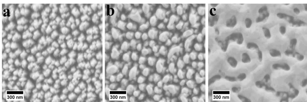
Figure 2. SEM micrographs of the sputtered Pt layer onto the porous columnar SDC films after annealing at 700 °C (2 h, air). With increasing Pt thickness from 5 nm (a) to 17 nm (b) and 50 nm (c), the Pt morphology changes from largely isolated particles to a highly porous, interconnected network.
