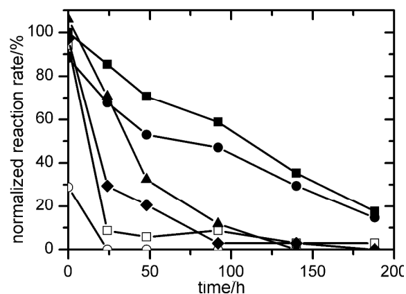
Fig. 3 Effect of mediators on laccase activity. Laccase activity was measured at intervals after incubation in the presence of no mediator (■), ABTS (●), TEMPO (▲), phenothiazine (◆), 4-hydroxybenzyl alcohol (□) or 2-hydroxybiphenyl (○). Reaction rates are expressed as a percentage of the rate in the control sample taken immediately after mixing laccase with buffer solution (no mediator, time = 0, V_0=0.112 \mu M s^{-1} ). All experiments were conducted in triplicate, and the standard deviation was less than 10% of the mean.
