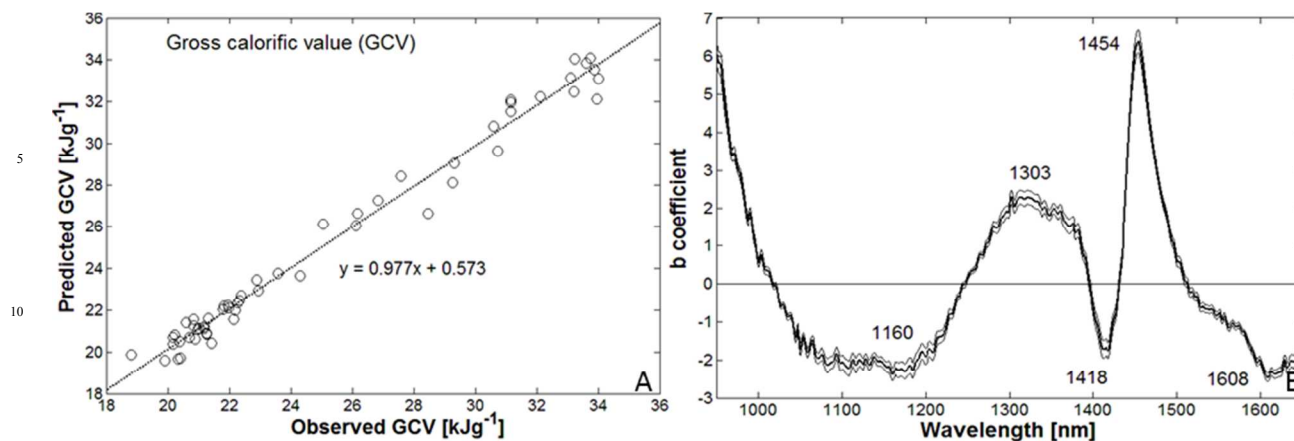
Fig. 5. A: Observed and predicted energy contents (gross calorific values, GCV) of raw and thermo-treated biomass. B: Model coefficients (average and \pm one standard deviation) for NIR based prediction of gross calorific values.
