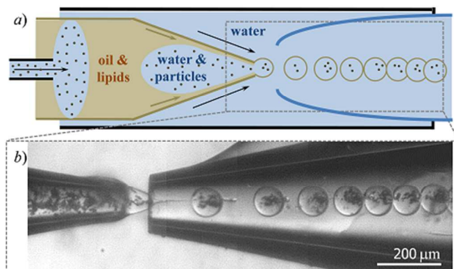
Figure 1. (a) Schematic illustration of the microfluidic device used to fabricate water-in-oil-in-water (W/O/W) double emulsion drops with ultrathin shells and P Si microparticles within their cores. (b) Optical microscope image of a typical production at flow rates of the inner, middle and outer phases of 700, 700, and 5000 \mu\text{L}/\text{h} , respectively.
