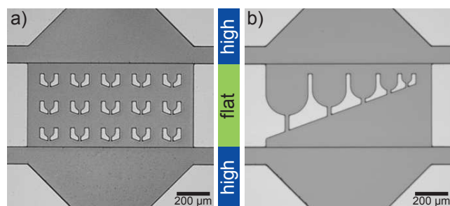
Fig. 1 Two-layer silicon wafer imaged with an upright microscope. (a) Device with trap diameter (corresponds to drop diameter) 55 \mu\text{m} (b) Device for drops of different diameter from 250 \mu\text{m} to 55 \mu\text{m} . The 'trap' region in the corresponding PDMS devices is flat compared to the rest of the device.
