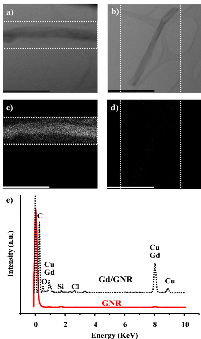
Fig. 2 TEM images of a) Gd/GNRs and b) GNRs. Electron dispersion spectroscopy (EDS) - TEM mapping for Gd^{3+} and Cu^{2+} of c) Gd/GNRs and d) GNRs (mapping areas designated by dotted white lines), and e) EDS spectra of the Gd/GNRs and GNRs (scale bars = 600 nm).
