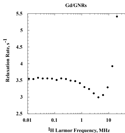
Fig. 5 The spin-lattice-relaxation normalized to Gd^{3+} concentration as a function of magnetic field strength reported as the ^1H Larmor frequency at 0.01 – 20 MHz and 25 ^{\circ}C for water protons in an aqueous suspension of the Gd/GNRs.
