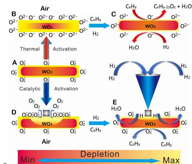
Fig.6 Schematic diagram of the charge transfer mechanisms of the TA and CA sensor. (A) WO 3 NPs in air at room temperature. (B) TA WO 3 NPs in air at high temperatures. (C) TA WO 3 NPs under hydrogen and hydrocarbon gases. (D) CA WO 3 NPs in air at room temperature. (E) CA WO 3 NPs under hydrogen and hydrocarbon gases at room temperature.
