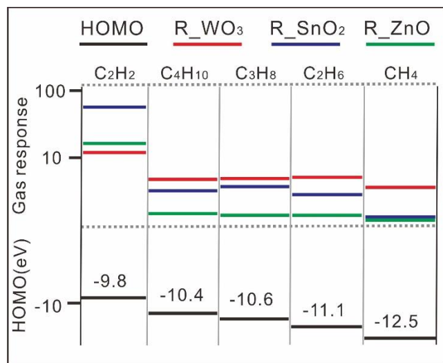
Fig.5 Gas-sensing responses of the three TA sensors to different hydrocarbon gases and the corresponding HOMO energy level obtained by DFT calculations.
