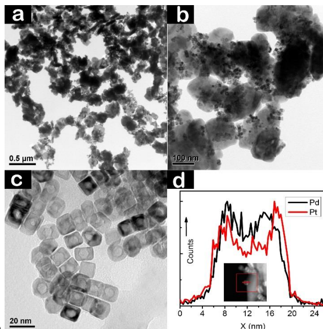
Fig.2 (a, b) TEM images of the Pt/Pd- \text{WO}_3 hybrid nanostructure. (c) High magnification TEM image of the hollow Pt/Pd NCs. (d) EDX line-scanning profile of a single Pt/Pd nanocube showing its hollow feature.
