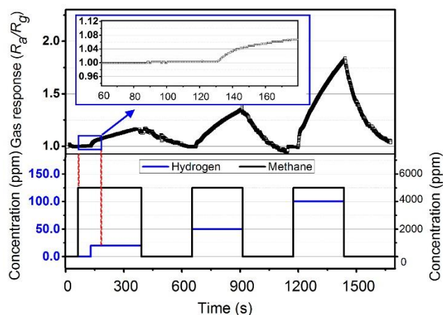
Fig.7 Dynamic response curve of the CA sensor to hydrogen in the presence of methane. The inset shows the real-time response of the sensor by introducing 5000 ppm methane at t=60 s and 20 ppm hydrogen at t=120 s.
