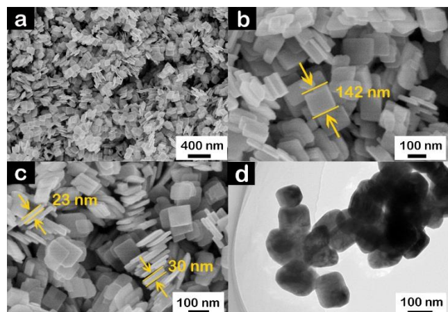
Fig.1 (a-c) SEM images of the \text{WO}_3 NPs. The representative width and thickness of the products are marked in (b) and (c), respectively. (d) A typical TEM image showing the dimensions of the \text{WO}_3 NPs.
