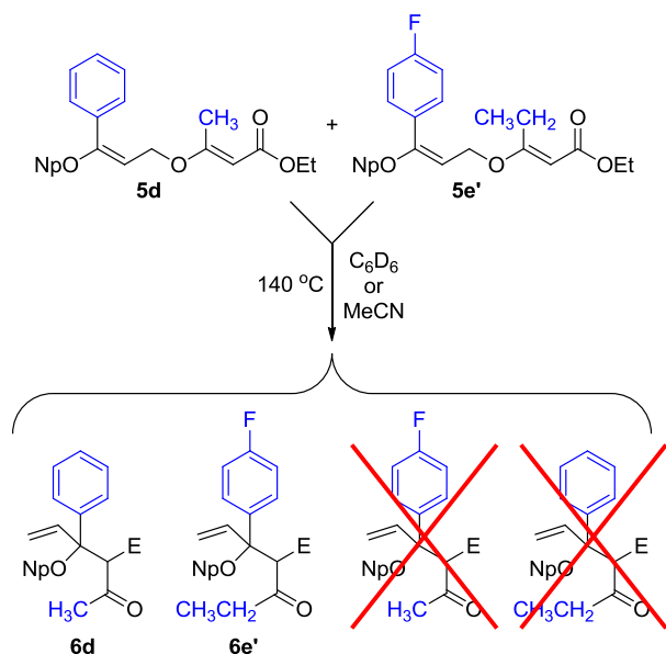
Scheme 3 Crossover experiment.
