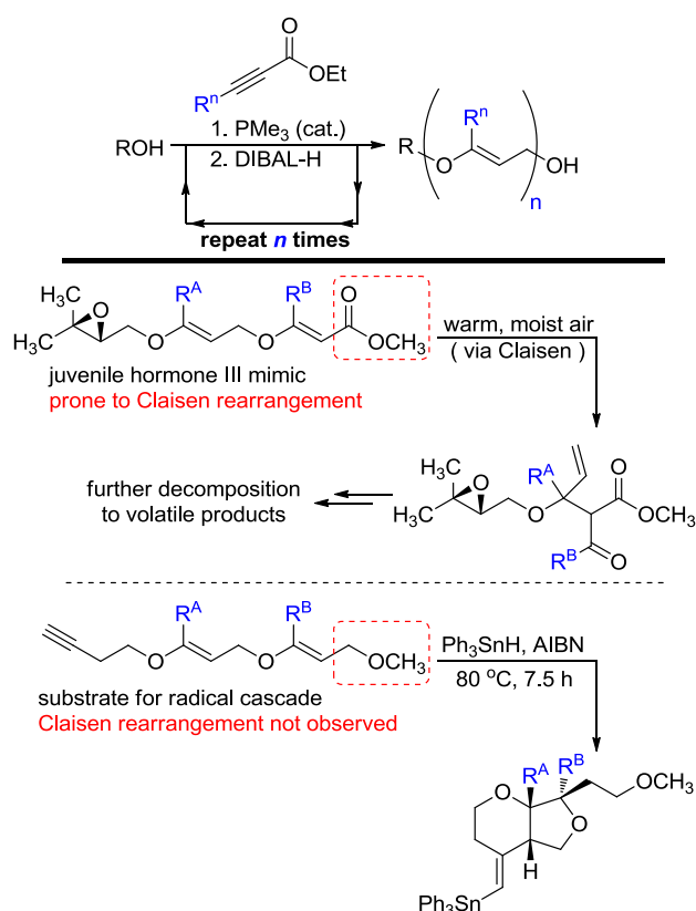
Figure 2 Iterative synthesis of oligo-vinyl ethers, and synthetic applications.
