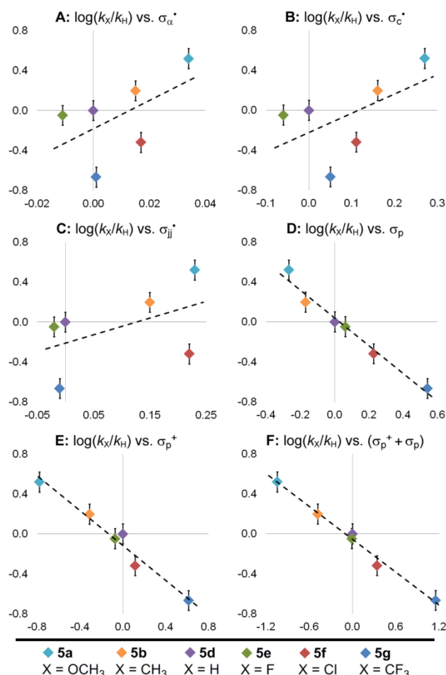
Figure 4. Hammett plots for the rate of rearrangement of compounds 5 , plotted against different \sigma values (derived from either polar or radical reactions) to probe mechanism.
