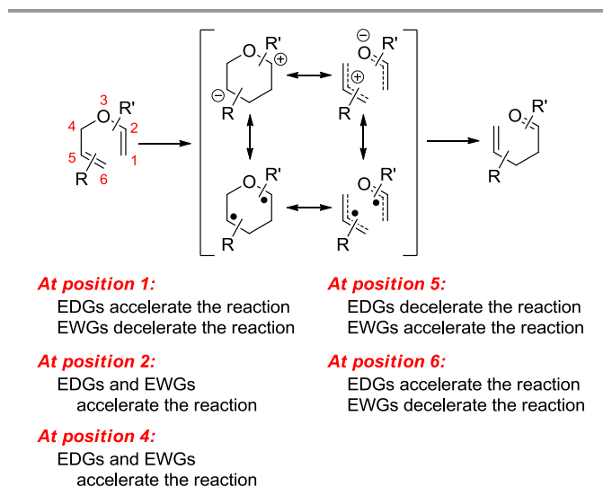
Figure 1 Mechanistic options for the aliphatic Claisen rearrangement, and a summary of known substituent effects.
