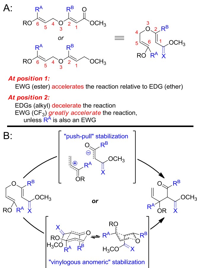
Figure 3 Reactivity of bis-vinyl ethers toward Claisen rearrangement. A: summary of Claisen rearrangement substituent effects observed from our earlier bis-vinyl ether studies; B: two plausible mechanistic possibilities for the rearrangement.
