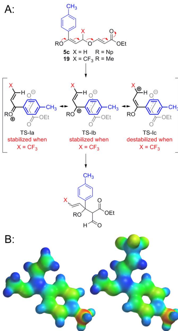
Figure 6 Rationale for transition state stabilization by the CF_3 substituent. A: Postulated resonance structures for the dissociative transition state. B: Calculated electronic potential maps for the cationic fragments of transition states leading from 5c and 19 .
