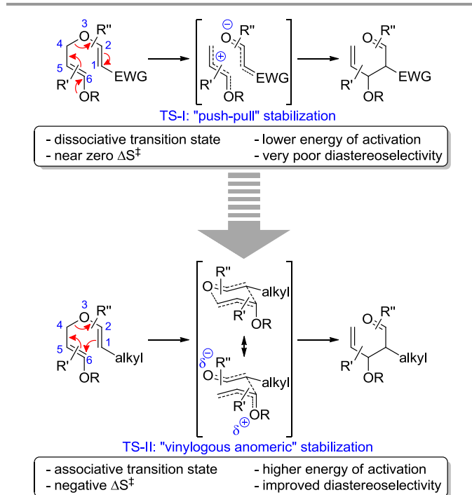
Scheme 4. Mechanistic proposal, accounting for differences in reactivity with different C-1 and C-6 substitution.
