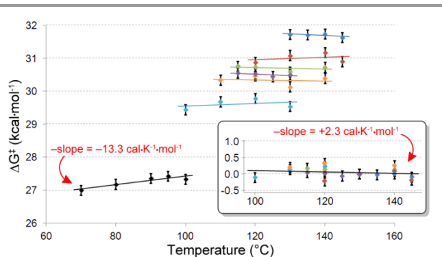
Figure 5 Change in \Delta G^\ddagger with temperature for bis-vinyl ethers 5 and 13 . Coloured data points correspond to measurements for compounds 5a–5g (see legend in Figure 4 for details). Black data points correspond to measurements for compound 13 . Inset plot shows the change in \Delta G^\ddagger (in units of \text{kcal}\cdot\text{mol}^{-1} ) for all aryl-substituted compounds, relative to the measured \Delta G^\ddagger at 130 °C. 65
