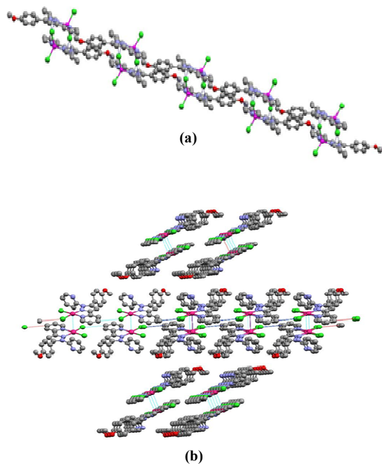
Fig. 12 (a) 1D chains parallel to the (1 0 1) direction for [\text{ZnCl}_2(\text{pypz}^{\text{R}(1)\text{py}})] (6) and (b) crossed in the (1 0 1) and (-1 1 0) for [\text{PdCl}_2(\text{pypz}^{\text{R}(1)\text{py}})] (11)
