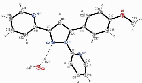
Fig. 5 ORTEP plot of [\text{pypz}^{\text{R}(1)\text{py}}]\cdot\text{H}_2\text{O} ( 1\cdot\text{H}_2\text{O} ) with 20% probability
