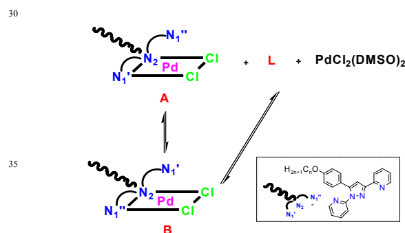
Scheme 2 Proposed equilibrium between A and B linkage isomers and the free ligand on DMSO-d 6 solution
