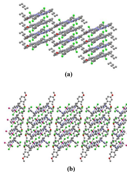
Fig. 13 Packings of (a) [\text{ZnCl}_2(\text{pypz}^{\text{R}(1)\text{py}})] (6) and (b) [\text{PdCl}_2(\text{pypz}^{\text{R}(1)\text{py}})] (11)
