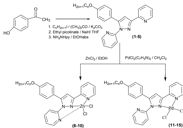
Scheme 1 Schematic synthesis of pypz R(n)py and [MCl 2 (pypz R(n)py )] (M=Zn, Pd)
