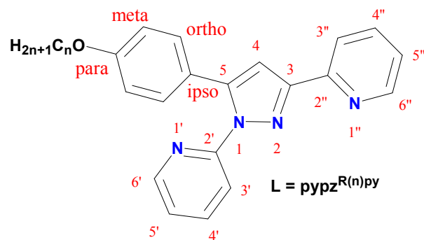
Fig. 1 Schematic representation and numbering of the atoms for pypz R(n)py ligands
