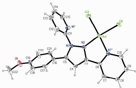
Fig. 9 ORTEP plot of [\text{PdCl}_2(\text{pypz}^{\text{R}(1)\text{py}})] \cdot \text{CH}_2\text{Cl}_2 ( 11 · \text{CH}_2\text{Cl}_2 ) with 20% probability. The dichloromethane molecule have been omitted for clarity
