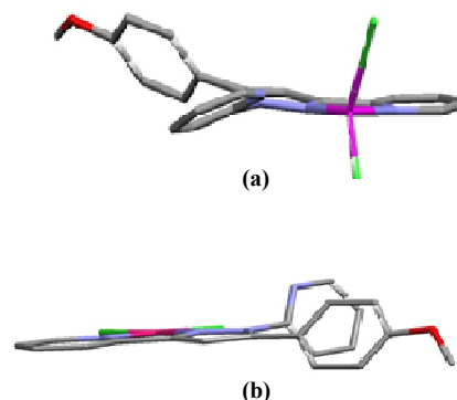
Fig. 10 View of the complexes (a) [\text{ZnCl}_2(\text{pypz}^{\text{R}(1)\text{py}})] ( 6 ) and (b) [\text{PdCl}_2(\text{pypz}^{\text{R}(1)\text{py}})] ( 11 ) showing the lack of planarity
