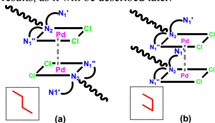
Fig.4 “Z”- (a) and “U”- (b) shaped binuclear isomers of [\text{PdCl}_2(\text{pypz}^{\text{R}(1)\text{py}})]
