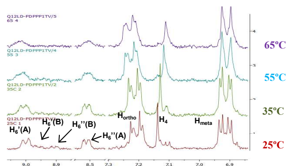
Fig. 3 Evolution of 1 H-NMR proton signals of [PdCl 2 (pypz R(1)py )] by increasing temperature
