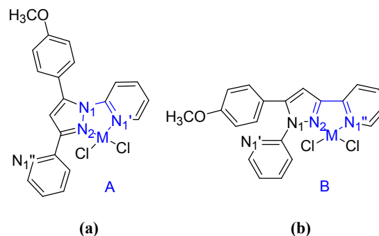
Fig. 2 Possible linkage isomers for [MCl 2 (pypz R(1)py )] (M=Zn, Pd)
