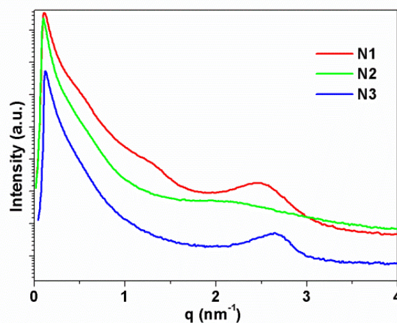
Fig. 3 Powder SAXS diffractogram of 2D networks N1-3 .
