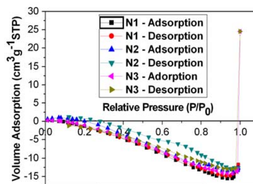
Fig. 4 Nitrogen adsorption-desorption isotherms of 2D networks N1-3 measured at 77.3 K.
