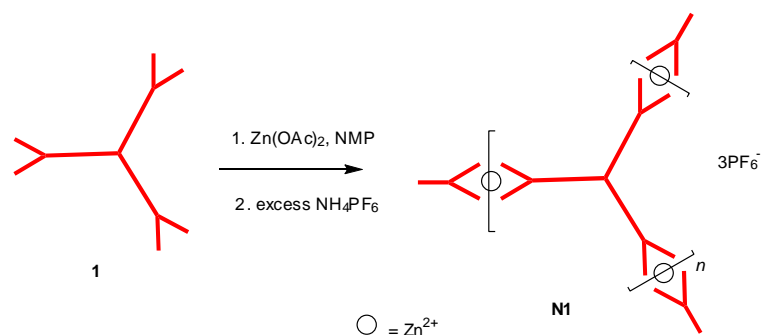
Scheme 5 Synthesis of one component 2D Zn 2+ co-ordinated self-assembled supramolecular network N1.
