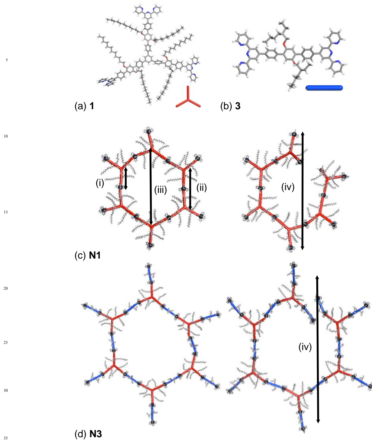
Fig. 5 The optimised geometry of (a) 1 and (b) 3 and idealised hexagons and broken hexagons for (c) N1 and (d) N3 respectively showing the four types of repeating distances potentially present within the extended network. The red rod inset in (a) represents 1 in the extended networks. The blue rod represents 3 in N3 . The black spheres represent the linking \text{Zn}^{2+} .
