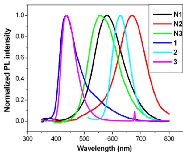
220 Fig. 8 Solid state photoluminescence spectra of core molecules 1 , 2 , 3 and their 2D self-assembled networks N1-3 .
