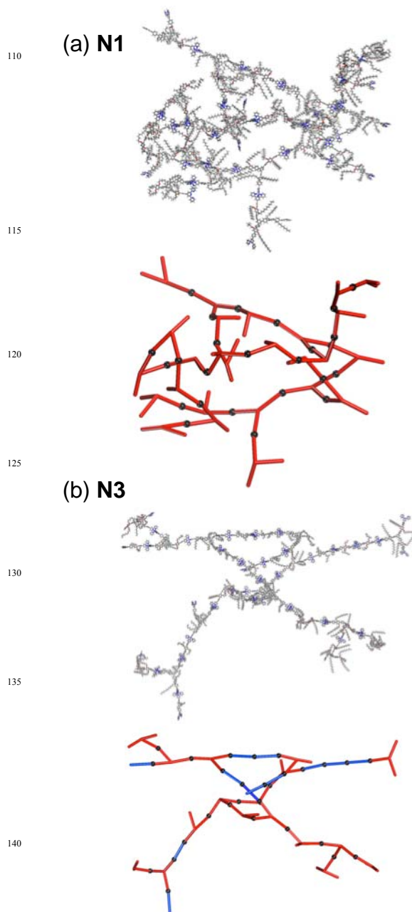
Fig. 6 Extended networks of (a) N1 and (b) N3 generated through an automated method with random choice of building block. Right – the network showing all atoms and, left – the underlying network with 1 and 3 represented as red and blue rods respectively. The black spheres represent the linking Zn^{2+} . The PF_6^- counter ions are omitted for clarity.
