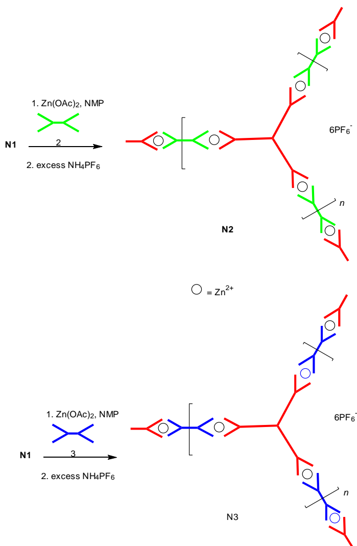
Scheme 6 Synthesis of 2D Zn 2+ co-ordinated self-assembled two component extended supramolecular networks N2 and N3.
