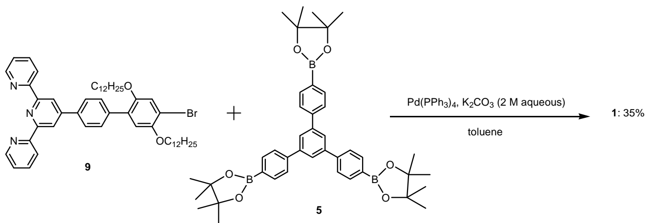
Scheme 4 Synthesis scheme of 2D supramolecule 1 .
