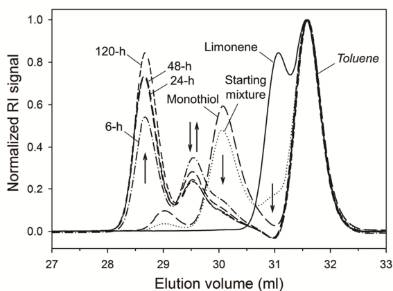
Figure 3. DMF-SEC elugram showing the development of mono- and di-addition products resulting from selective thiol-ene coupling of 1 with 2 under thermal reaction conditions. The small bands centered at 29 ml represent trace amounts of disulfide product. The flow-rate marker (toluene) was set at 31.5 ml. Arrows denote directions in consumption and/or formation.
