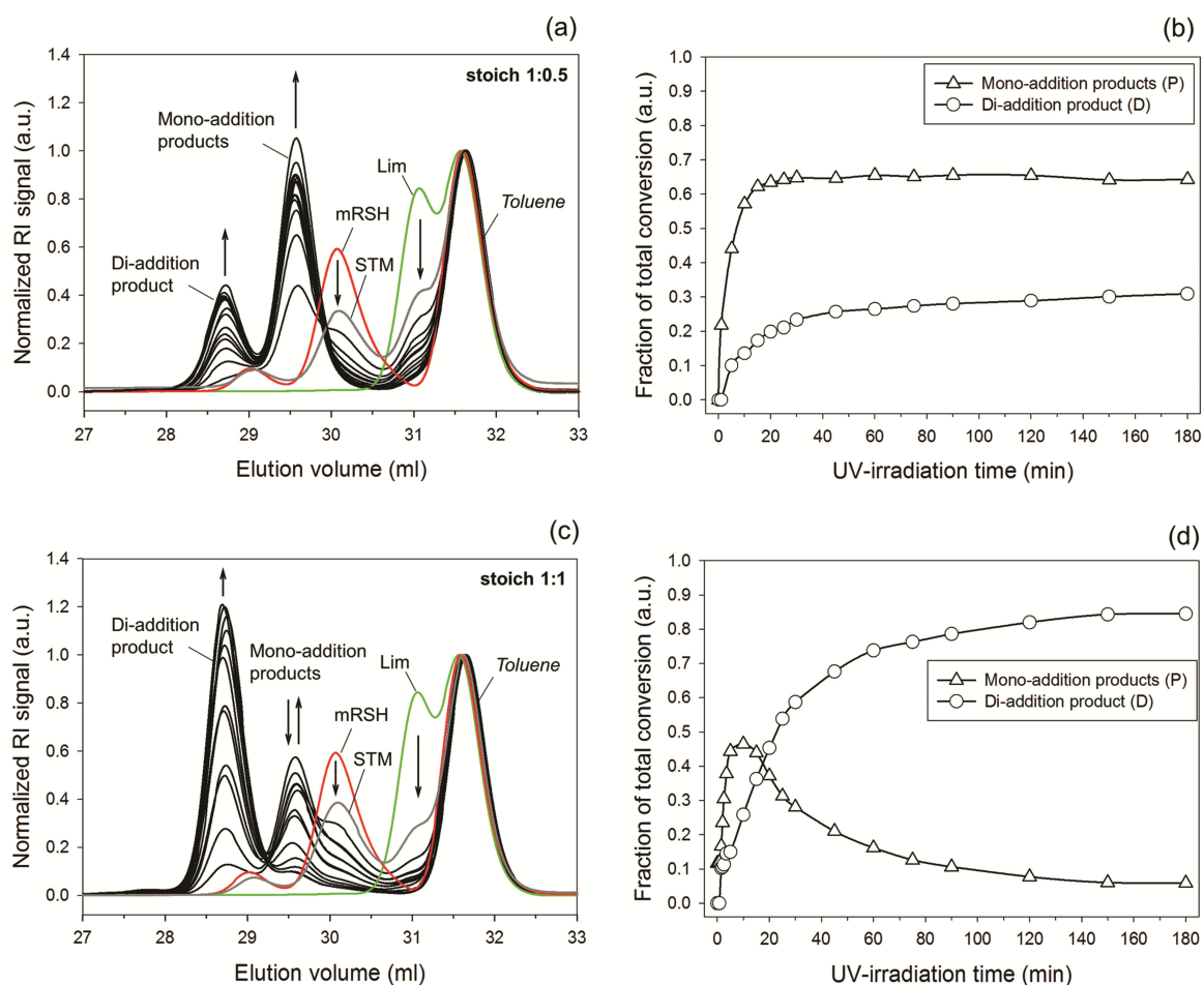
Figure 7. Normalized DMF-SEC elugrams (left side) and corresponding kinetic profiles (right side) showing the time-course evolution of mono- ( 3 + 4 = P ) and di-addition ( 5 = D ) products resulting from selective thiol-ene coupling under photochemical reaction conditions using two different stoichiometries with respect to reactive functional groups: (a) and (b) 1:0.5 mole ratio (1:1 thiol-terpene molecular ratio); (c) and (d) 1:1 mole ratio (2:1 thiol-terpene molecular ratio). Starting thiol-ene mixture (STM, grey line); Limonene (Lim 1, green line); and, Monothiol (mRSH 2, red line). The small bands centered at 29 ml represent trace amounts of disulfide product. The flow-rate marker (toluene) was set at 31.5 ml. Arrows denote directions in increase or decrease of the given coupled product(s).
