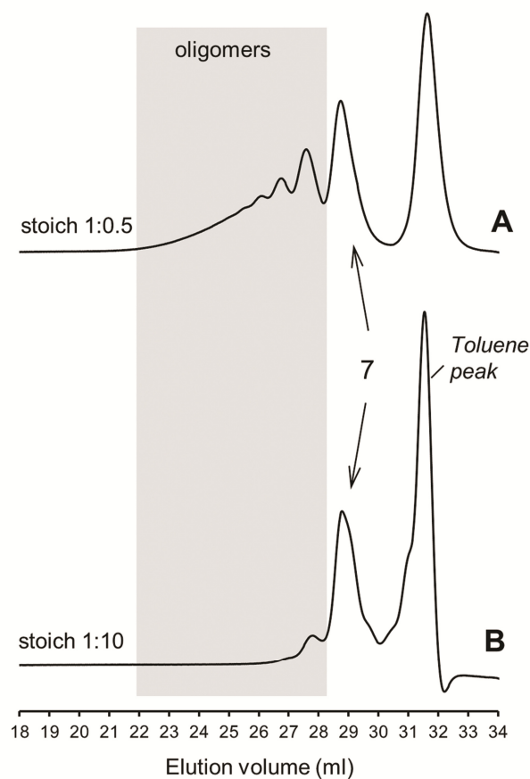
Figure 9. Qualitative DMF-SEC elugrams for the multifunctional system based on the photoinitiated reaction of ( R )-(+)-limonene ( 1 ) with TMP-trimercaptopropionate ( 6 ) using two different thiol-to-ene stoichiometries. In elugram B the small band shoulders located at 29.5, 30.5 and 31.0 ml represent vestigial amounts of partially coupled products, unreacted trithiol and limonene, respectively. Thiol:Ene = x:y (functional group stoichiometry). Shaded grey region denotes occurrence of high molecular weight ‘hyperbranched-like’ oligomers.
