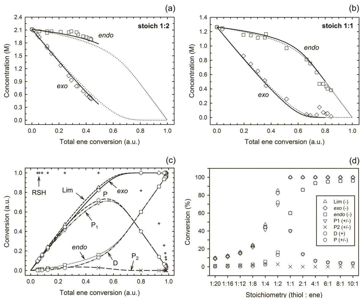
Figure 8. Concentration–conversion plots a/b and evolution of conversion as a function of total ene conversion or thiol–ene stoichiometry c/d. Experimental (symbols) vs. simulated (lines) data for a composition mole ratio of (a) 1:2 ( i.e. , 1:0.5), and (b) 1:1 with respect to thiol–ene functionalities. (c) general simulation chart covering a stoichiometry range of 1:20 \leq \text{thiol:ene} \leq 10:1 . Full-range plot-lines represent a maximal thiol–ene stoichiometry of 20:1. (d) effect of stoichiometry on the final conversion of variables. Individual symbols as data points in plots (c) and (d) denote final computed concentrations or conversions (at t = 180 min) of each variable at a given initial thiol–ene stoichiometry. [\text{DMPA}]_0 = 0.07 M ( \sim 2.0 wt.% of total amount of reactants) in all simulations. Symbols (+) and (–) in plot (d) denote positive or negative conversions of a given variable, respectively.
