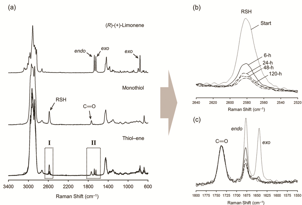
Figure 2. FT-Raman spectra collection showing the time-evolution of thiol and ene functional groups from a starting 1:1 stoichiometric mixture composed of ( R )-(+)-limonene ( 1 ) and iso -tridecyl 3-mercapto propionate ( 2 ). (a) overall spectra in comparison to the individual pure compounds; (b) enhancement of region I showing the depletion of thiol (2573 cm -1 ); and, (c) zoom-in of region II showing the disappearance of unsaturations with favored coupling at the exocyclic double-bond position (1645 cm -1 ). The carbonyl moiety (C=O, 1735 cm -1 ) was used as internal reference band in the spectral normalization process (only for the thiol-ene spectra).
