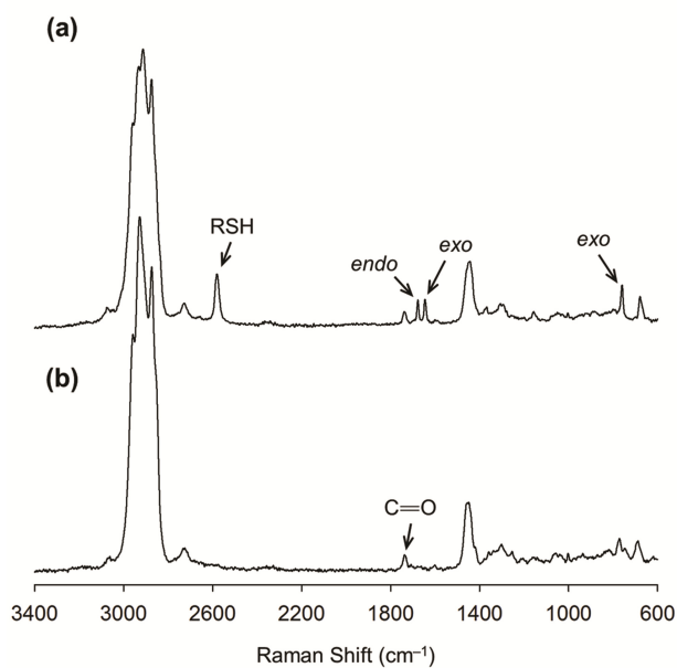
Figure 6. Normalized FT-Raman spectra of samples obtained from photoinduced thiol-ene reaction of monofunctional system mixed on a 1:1 thiol-ene functional group stoichiometry. (a) before reaction (starting mixture at time zero); (b) after a reaction period of 8-hours conducted at room temperature. The carbonyl ester group ( \text{C}=\text{O} , 1735\text{ cm}^{-1} ) was used as internal reference band in the spectral normalization process.
