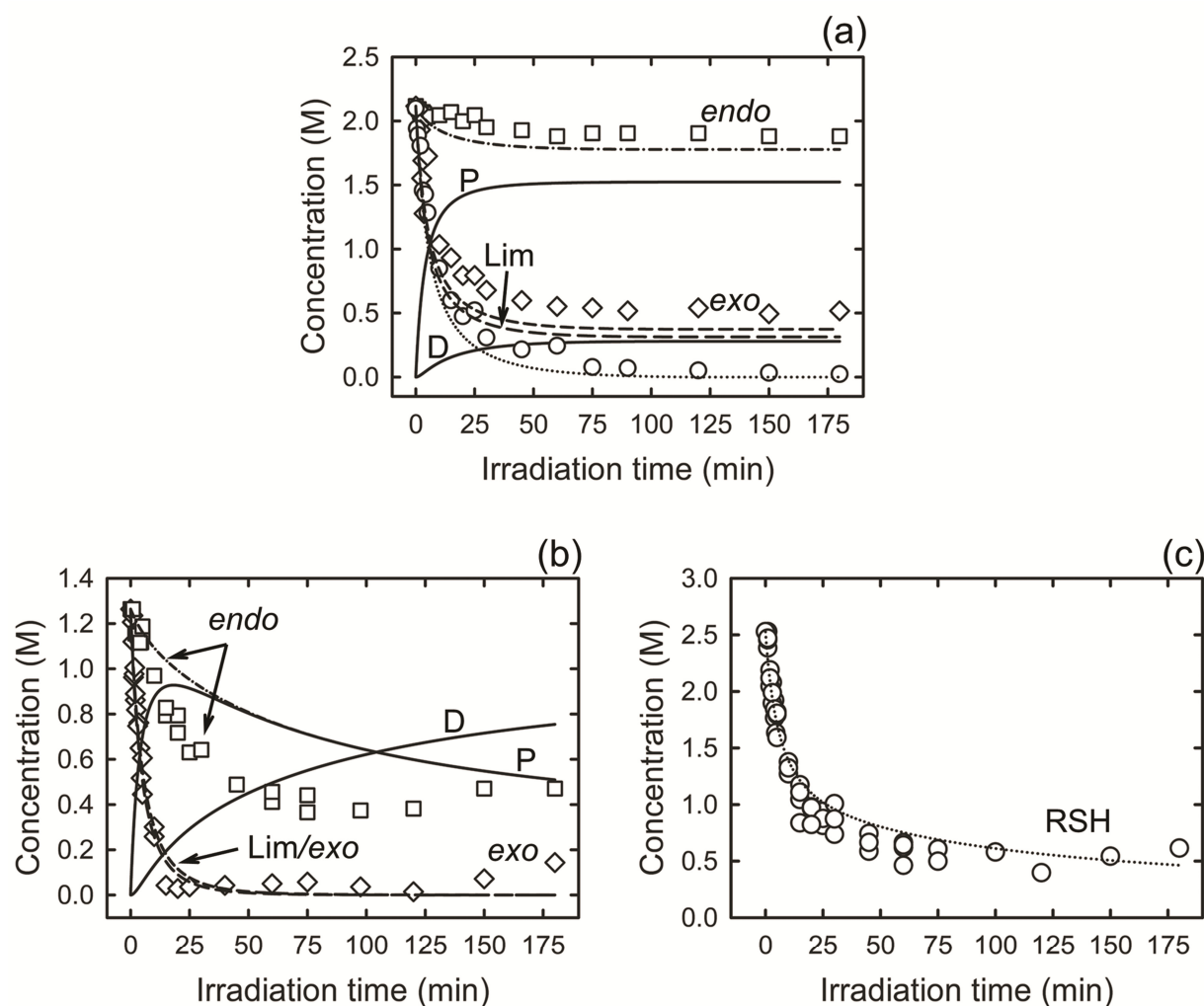
Figure 4. Kinetic plots of experimental (symbols) vs. simulated model predictions (lines) as a function of initial thiol–ene stoichiometry obtained from photoinduced reactions of the monofunctional system. (a) stoichiometry of 1:0.5, (b) and (c) stoichiometry of 1:1. Stoichiometric mole ratios are reported with respect to thiol and ene functionalities. Legend: thiol (RSH; ○, dotted line), limonene (Lim; long-dashed line), endocyclic unsaturation ( endo ; □, dashed-dotted line); and, exocyclic unsaturation ( exo ; ◇, medium-dashed line). Mono- (P) and di-addition (D) products are depicted by the continuous solid lines. Temporal evolution of overall alkene functional groups ( i.e. , enes present both in limonene and di-addition products) were calculated as: [exo]_t = [Lim]_t + [P_2]_t and [endo]_t = [Lim]_t + [P_1]_t from computed limonene and individual mono-additions.
