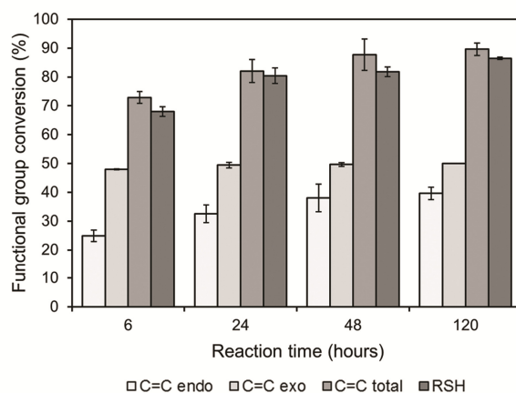
Figure 1. Extent of functional group conversion for a reaction mixture comprised of limonene ( 1 ) and iso -tridecyl 3-mercaptopropionate ( 2 ) reacted on a 1:1 mole stoichiometry with respect to thiol-ene functional groups, as provided by ^1\text{H} NMR (double-bonds) and FT-Raman (thiol). The reactions were conducted thermally with 2.0 wt.% of AIBN in bulk at \sim 70^\circ\text{C} in the absence of oxygen. Error bars represent one standard deviation about the mean value measured from three independent reactions.
