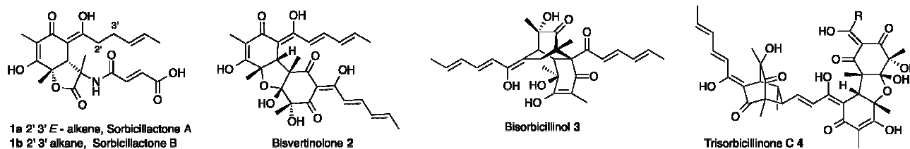
Figure 1. Structural diversity among the sorbicillinoid family. R = CH=CHCH=CHMe
