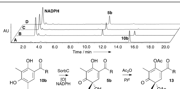
Scheme 3. Conversion of dihydrosorbicillin 10b to dihydrosorbicillinol 5b and its acetylation. DAD HPLC traces (200 - 400 nm): A , 0 min (before addition of NADPH); B , 10 min; C , 20 min; D , 30 min. R = CH 2 CH 2 CH=CHCH 3
