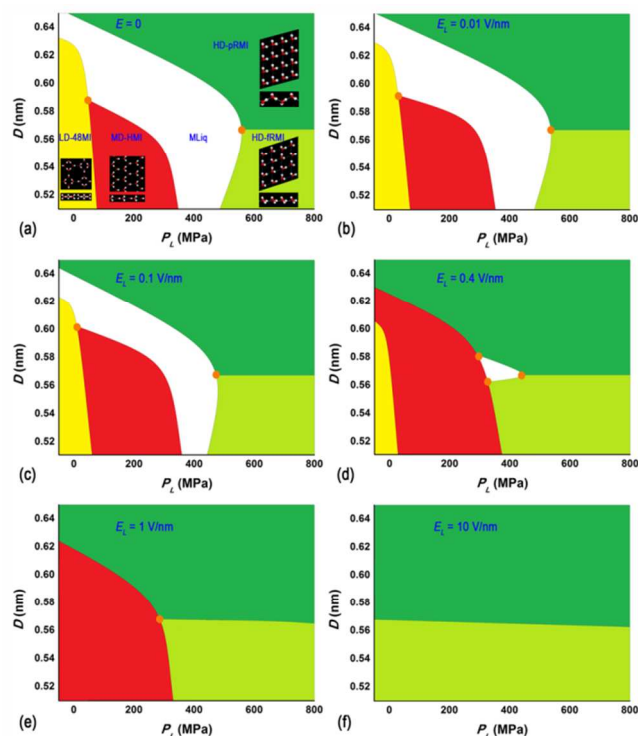
Fig. 3. Semi-quantitative phase diagrams of monolayer water confined between two hydrophobic walls at 200 K with the lateral electric field strength E_L = (a) 0, (b) 0.01, (c) 0.1, (d) 0.4, (e) 1.0, and (f) 10 V/nm, respectively. Triple points are highlighted by orange circles.
