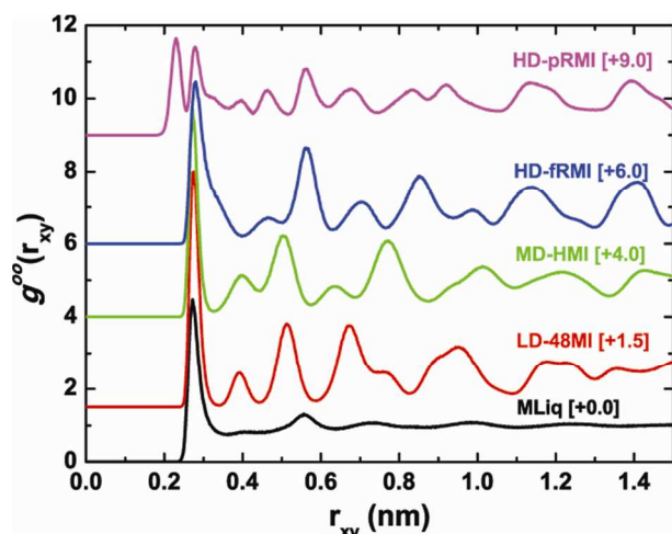
Fig. 6. Lateral oxygen-oxygen radial distribution functions g^{oo}(r_{xy}) at T = 200 K for MLiq ( P_L = 400 MPa, D = 0.557 nm), LD-48MI ( P_L = -50 MPa, D = 0.557 nm), MD-HMI ( P_L = 100 MPa, D = 0.557 nm), HD-fRMI ( P_L = 600 MPa, D = 0.52 nm), and HD-pRMI ( P_L = 600 MPa, D = 0.64 nm), respectively.
