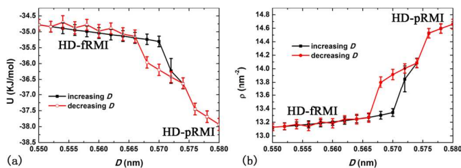
Fig. 9. The potential energy U (a) and area density \rho (b) at P_L = 800 \text{ MPa} and T = 200 \text{ K} with increasing D first, followed by the decreasing D process.
