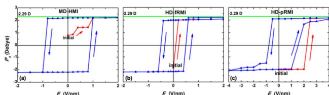
Fig. 7. Hysteresis loops of polarization, P_x , per water molecule for MD-HMI, HD-fRMI, and HD-pRMI. The electric field E was applied along the X axis. The
