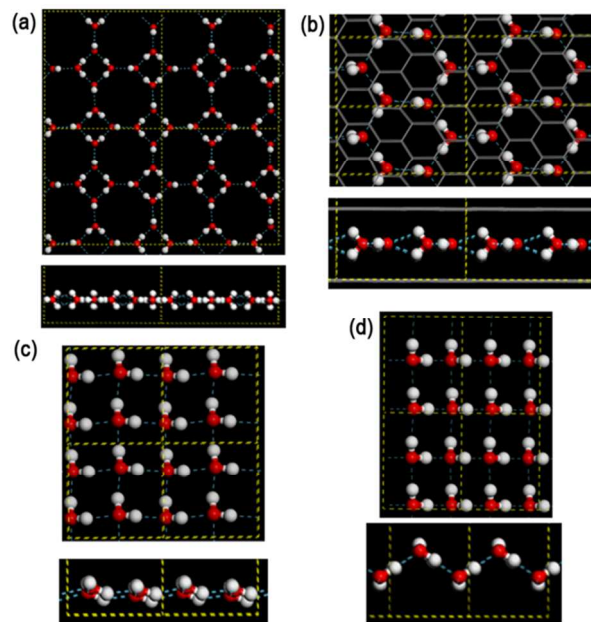
Fig. 8. The optimized structures of monolayer ices (upper panel: top view; lower panel: side view) (a) LD-48MI ( L_x = 13.46 Å, L_y = 13.46 Å), (b) MD-HMI confined between two graphene layers ( L_x = 8.67 Å, L_y = 4.62 Å), (c) HD-fRMI ( L_x = 5.52 Å, L_y = 5.5 Å), and (d) HD-pRMI ( L_x = 5.62 Å, L_y = 4.62 Å). L_x and L_y are lattice constants of the supercell. Yellow dashed lines illustrate the boundary of the supercell. Blue dashed lines represent hydrogen bonds among water molecules. Gray lines in (b) represent the graphene layers.
