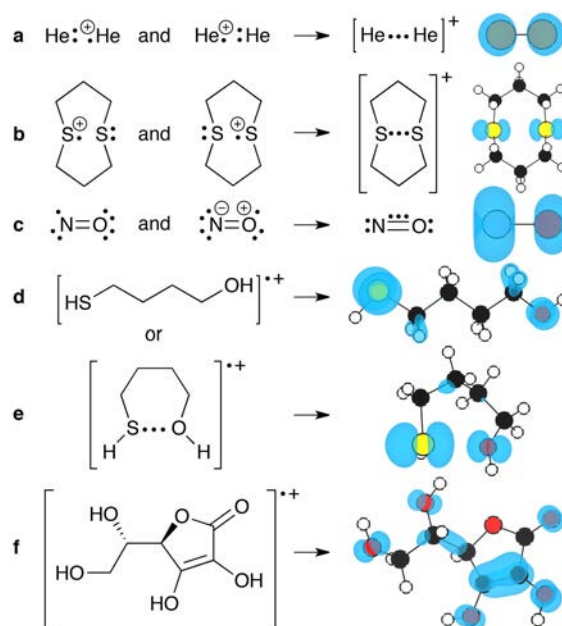
Fig. 1 Examples of three-electron two-centred systems: a) \text{He}_2^+ ; b) 1,5-dithiocane cationic radical; c) NO neutral radical. The hydroxy-thiol cationic radical shown in d/e can exist in multiple conformations, the straight-chain (d) and the pseudo-cyclic (e). As the system complexity increases, so does the description of the radical localisation; an example is the cationic ascorbic acid radical, f. Calculated spin density ( \rho^\uparrow - \rho^\downarrow ) for each radical state is shown on the right.
