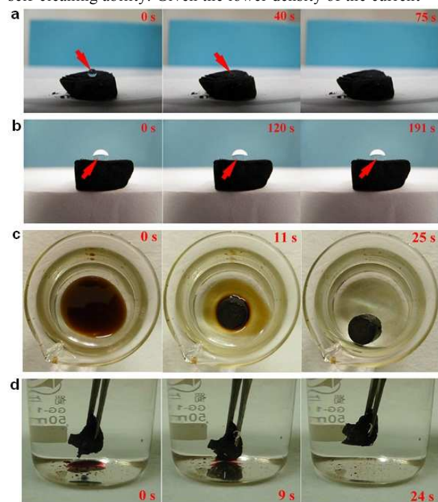
Figure 3. Water and oil absorption of graphene sorbent. Series of digital photos showing the water / organic chemicals absorption by the graphene sorbent. a) A water drop was completely absorbed by SG-R (without soot treatment) after 75 seconds; b) SG-F, the sorbent treated with candle soot, shows excellent water resistance, indicating that the carbon nanoparticles generated by the soot play a critical role on deciding the performance of the spongy graphene; c) The SG-F absorbs crude oil (dark brown, thick liquid) floating on the water; d) The SG-F absorbs phenixin (dyed with red color) from the bottom of the water.
