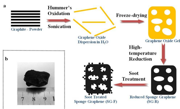
Figure 1. Fabrication and macroscopic appearance of spongy graphene (SG). a) Fabrication of SG. The components are intentionally drawn not into scale. b) Macroscopic image of SG bulk.
