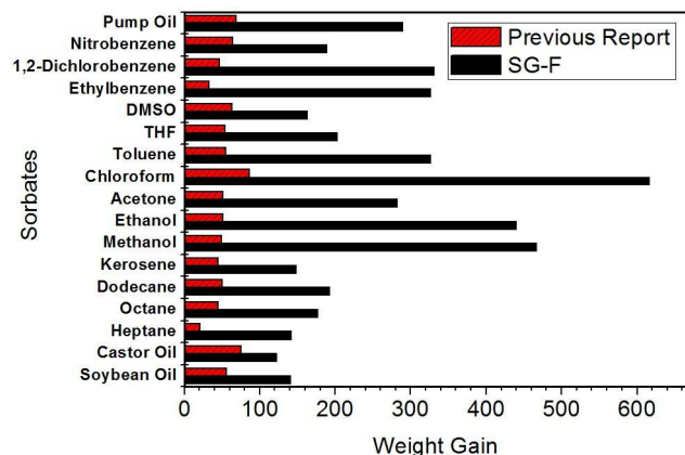
Figure 4. The capacity of graphene sorbent towards various organic chemicals. Absorption capacity of SG-F, the soot-treated graphene sorbent, towards various organic chemicals. Black bars: performance of SG-F studied in this report. Red bars: corresponding performance of SG prepared elsewhere. 12 A maximum of 616 times of the own weight of graphene sorbent can be absorbed when using chloroform as the target substance, which is ~ 8 times higher than previous report.
