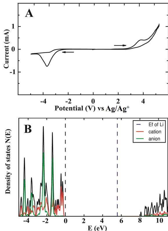
Figure 3. (A). Cyclic voltammograms of \text{PP}_{13}\text{PF}_6 at 100 °C. Third cycle is shown. (B) Calculated density of states of \text{PP}_{13}\text{PF}_6 .
