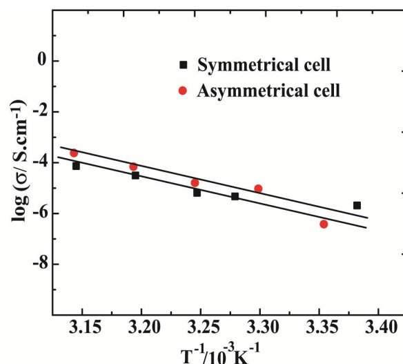
Figure 5. Arrhenius plot of Li-ion conductivity in the symmetric and asymmetric cells of the \text{PP}_{13}\text{PF}_6 ionic crystal.
