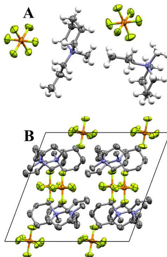
Figure 2. X-ray crystal structure of PP 13 PF 6 at 223 K (50% thermal ellipsoids): (A) asymmetric unit (hydrogens as fixed spheres of radius 0.30 Å) (B) unit cell viewed along the b -axis (hydrogens omitted for clarity)
