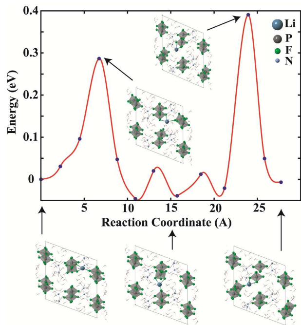
Figure 6. The minimum energy path for Li-ion diffusion in \text{PP}_{13}\text{PF}_6 .
