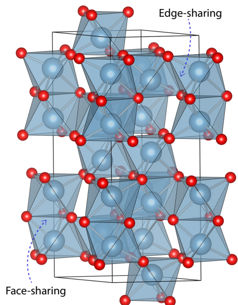
Fig. 1 Face-sharing and edge-sharing \text{AlO}_6 octahedral units in the corundum structure of \text{Al}_2\text{O}_3 (hexagonal crystal). The two sets of oxide ligands in the trigonal antiprismatic geometry ( D_{3d} symmetry) are shown.
