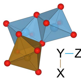
Fig. 5 Illustration of a \text{Ti}^{\text{III}}-(\text{Ti}^{\text{IV}} - \text{Fe}^{\text{II}}) tri-cluster. The L-shaped geometry of metal tri-clusters is shown, where X-Y are edge-sharing and Y-Z are face-sharing. The notation X-(Y-Z) is used in Table 10.
