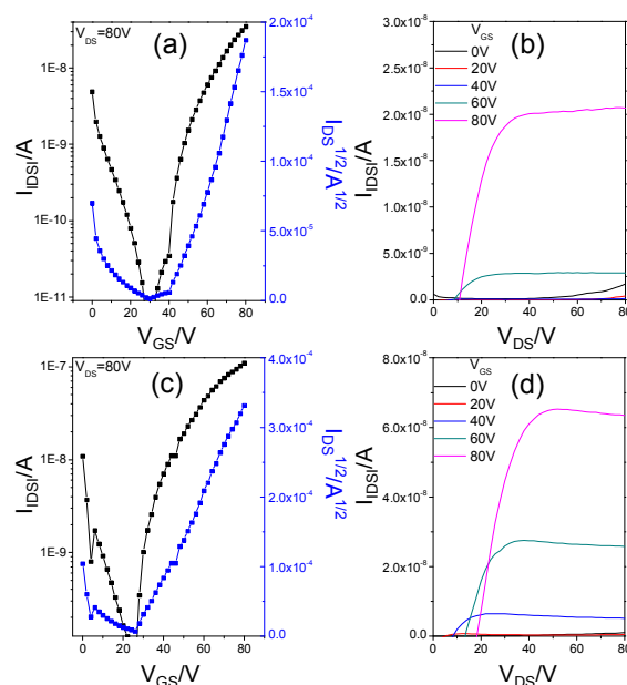
Figure 7. Transfer and output curves of OTFT devices with P1 (a and b) and P2 (c and d) thin films annealed at 150 °C for 20 min. Device dimensions: channel width ( W ) = 1 mm; channel length ( L ) = 30 \mu\text{m} .
