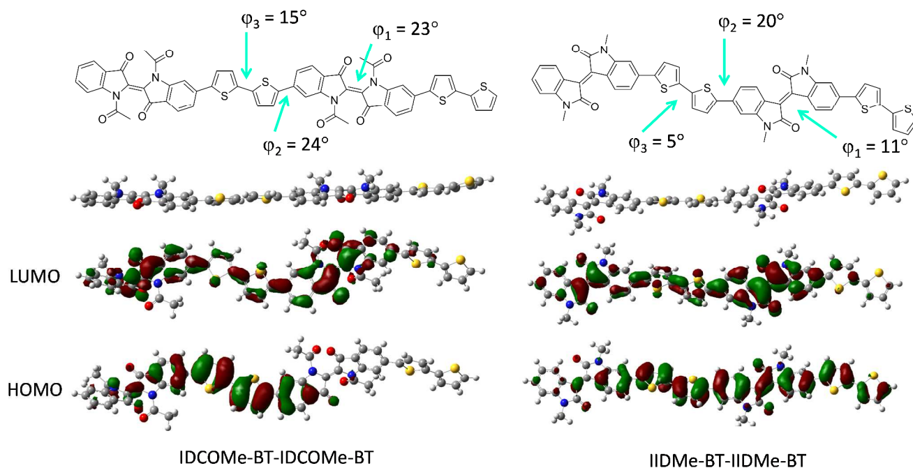
Figure 2. The chemical structure, geometry, LUMO orbital, and HOMO orbital of two model dimers IDCOMe-BT-IDCOMe-BT and IIDMe-BT-IIDMe-BT, which correspond to acyl-substituted PIDBT ( P1 or P2 ) and alkyl-substituted PIIDBT, 27 respectively, obtained by performing density functional theory (DFT) calculations with B3LYP 6-31G* basic set.
