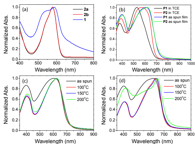
Figure 3. UV-vis absorption spectra of (a) 1 , 2a and 2b in TCE solutions; (b) P1 and P2 in TCE solutions and in thin films; (c) P1 and (d) P2 thin films on glass substrates annealed at different temperatures.
