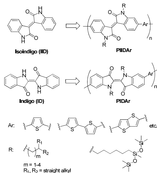
Figure 1. Structures of isoindigo (IID) and indigo (ID) and their polymers.
