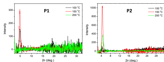
Figure 5. XRD diagrams obtained from spin-coating P1 and P2 thin film on silicon substrates annealed at 100, 150 and 200 °C.
