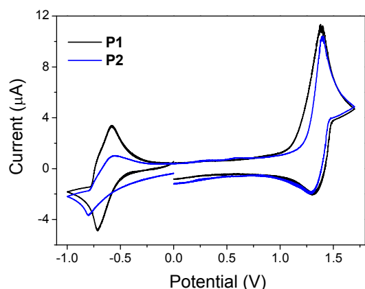
Figure 4. Cyclic voltammograms of as-spun P1 and P2 thin films measured in anhydrous \text{CH}_3\text{CN} solution using \text{Bu}_4\text{NPF}_6 as the electrolyte.
