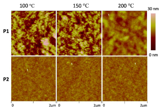
Figure 6. AFM images ( 2 \mu\text{m} \times 2 \mu\text{m} ) of P1 and P2 thin films ( \sim 50 – 60 nm) spin coated on silicon substrate annealed at 100, 150 and 200 °C under nitrogen.
