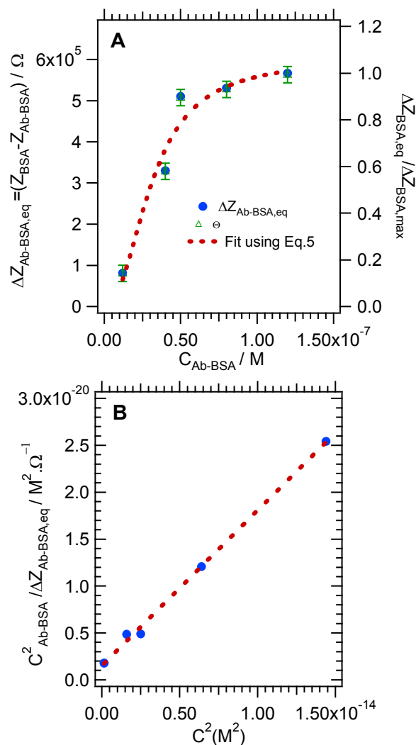
Figure 3. Calibration curve obtained for various Ab-BSA concentration loaded on the coated PET surface with BSA. (A) An association isotherm of Ab-BSA on the adsorbed BSA obtained from various experimental sensorgrams from 12 nM to 120 nM concentration. (B). Linearization step of the association isotherm using a linear fit as indicated in equation 7.
