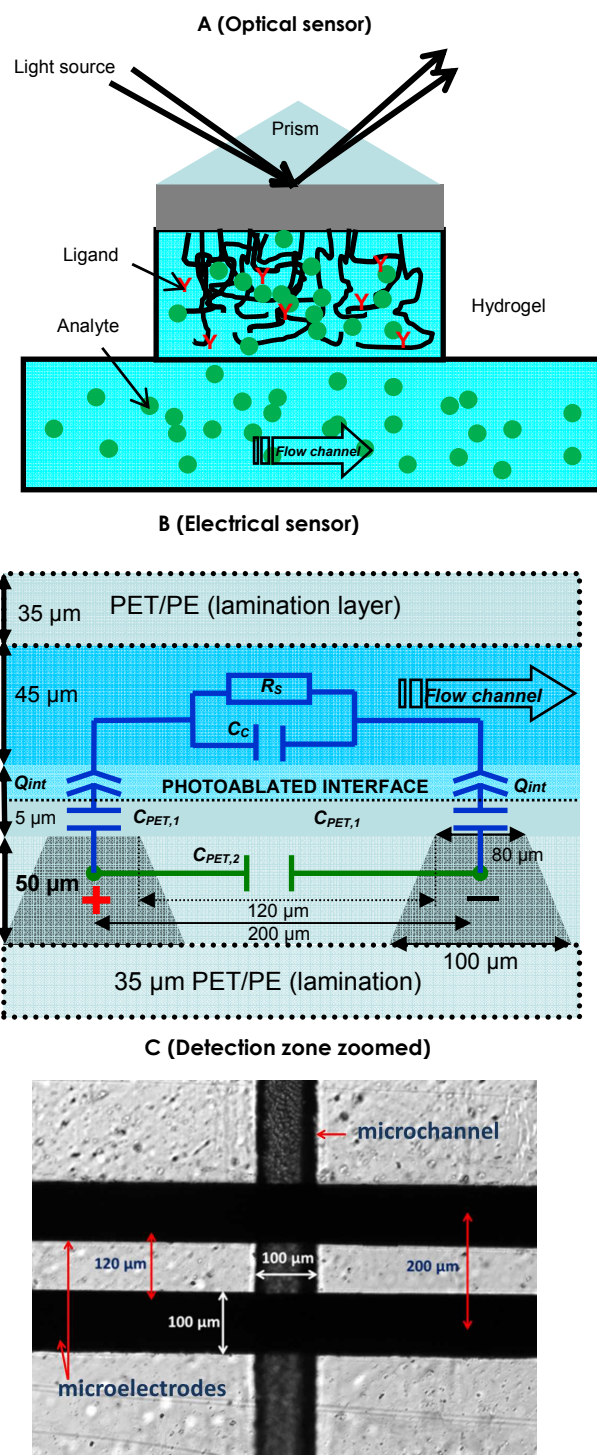
Figure 1. A. Schematic representation of the BIACORE optical biosensor. The hydrogel is 100 nm high approximately; the flow channel for a standard instrument is 24 mm long, 50 \mu m high and 500 \mu m width. The ligand is immobilised in the hydrogel, the analyte flows in the channel and diffuses in the gel where it binds to the ligand. B. Cross section of the dielectric interface microelectrode/ PET/ microchannel and the corresponding electrical equivalent circuit: C_{PET,2} for the 120 \mu m-PET layer impedance (distance separation), C_{PET,1} for the 5 \mu m-PET layer impedance (non-contact layer thickness), the element CPE, Q_{int} , for the interfacial impedance (photoablated surface), and the parallel association of the solution resistance, R_s , and the cell capacitance, C_c . Please note
