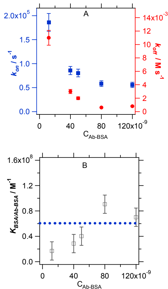
Figure 5. Kinetic parameters obtained from the fitted sensorgrams of interfacial impedance modulus with several Ab-BSA (from 1.2 \times 10^{-8} to 1.2 \times 10^7 ) loaded in the flow microchannel sensor coated with BSA. A. The values obtained were from fitting procedure using equation 12 leading k_{on} and k_{off} parameters which appear on left-axis and right-axis, respectively. B. The equilibrium constant corresponding to each k_{on} / k_{off} ratio is indicated for each Ab-BSA concentration (See Table 2 in the supplementary material).
