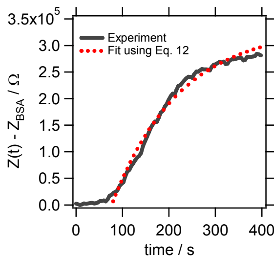
Figure 4. Experimental and fitted sensorgram of interfacial impedance modulus for 4 \times 10^{-8} M of Ab-BSA loaded in the flow microchannel sensor showing the association reaction between Ab-BSA and the adsorbed BSA at a fixed frequency of 400 Hz and for a flow rate of 7.2 \mu L \text{ min}^{-1} . The curve fit was performed with equation 12 leading k_{on} , k_{off} equal to 8.56 \times 10^4 s^{-1} and 3 \times 10^{-3} M s^{-1} , respectively.
