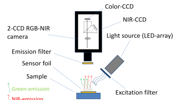
Fig. 2 Schematic drawing of the imaging set-up.
