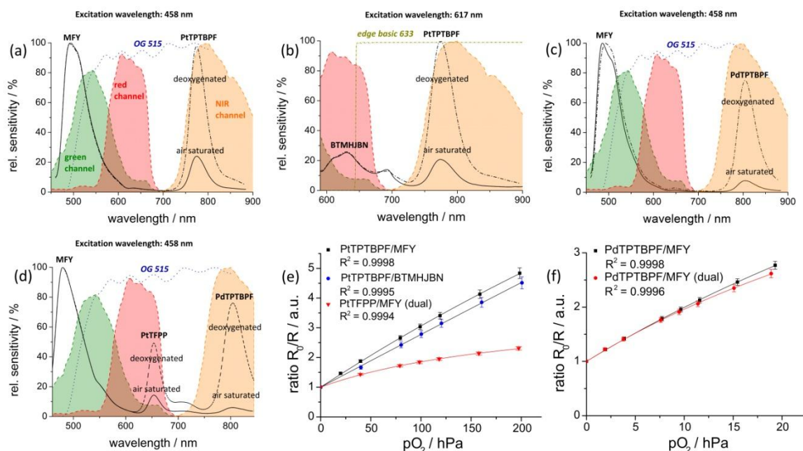
Fig. 5 Spectral properties (a-d) of the oxygen imaging set up at deoxygenated and air saturated conditions; shown are the spectral sensitivity of the camera channels, the emission spectra of the dye systems PtTPTBPF/MFY (a), PtTPTBPF/BTMHJBN (b), PdTPTBPF/MFY (c) and PtTFPP/MFY/PdTPTBPF (d) and the spectra of the emission filters (OG 515 and edge basic 633). Stern-Volmer calibration curves (e-f) for the oxygen optodes at 25°C. Lines indicate a fit according to equation 1.
