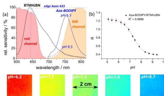
Fig. 7 Spectral properties of the pH imaging set-up at pH 5.5 and 9.5 (a); shown are the spectral sensitivity of the camera channels, the emission spectra of the used dyes (BTMHJBN and Aza-BODIPY) and the spectrum of the emission filter (edge basic 633); calibration curve (b) for the pH optode at 25 °C. Lines indicate a fit according to equation 2. Below: Pseudo colour images of the referenced images of the pH sensor film at different pH values.
