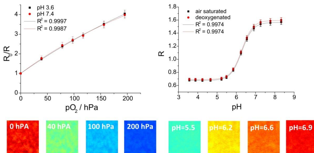
Fig. 9 Above: Calibration curves of the dual-parameter oxygen/pH sensor at 21 °C. Lines indicate a fit according to equations 1 and 2. Below: Pseudo colour images of the dual-parameter oxygen/pH sensor at certain oxygen concentrations and pH values.
