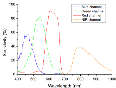
Fig. 3 Spectral response of the camera and the 4-channels adapted from Jai ( www.jai.com ).
