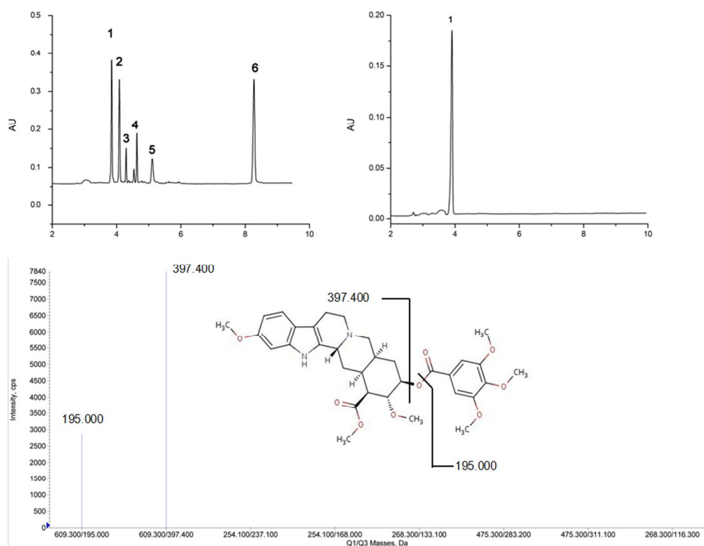
Fig. 4 The electropherograms of a tonic wine sample (top right) and a mixed standard solution (top left) with the mass spectrum of RSP (below). Peak indentifications: 1-RSP, 2-CTD, 3-IDP, 4-HCT, 5-NDP, 6-VST. 253x204mm (96 x 96 DPI)
