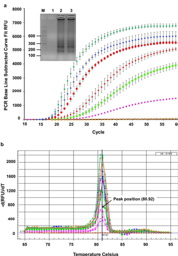
Figure 1 Real-time fluorescent CPA with different concentrations of pullulan. Pullulan concentrations: green triangle, 1 % (w/v); blue diamond, 0.5 % (w/v); red square, 2 % (w/v); red diamond, pullulan-free (control group); green square, 4 % (w/v); pink diamond, 5 % (w/v); brown triangle, no template control. a) Amplification curves of T-Nos transcript. Error bars, SD. Inside shows gel electrophoresis for CPA products after amplified for one hour. M is DNA marker
