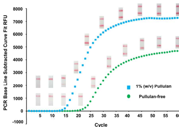
Figure 3 Time corresponding combination of real time fluorescent CPA and LFD assay on 1 % (w/v) concentration of pullulan system (blue line) and pullulan-free condition (green line). The CPA products were taken out for LFD detection respectively at end point of 5, 10, 15, 20, 25, 30, 35, 40, 50, 60 minute of DNA amplification.
