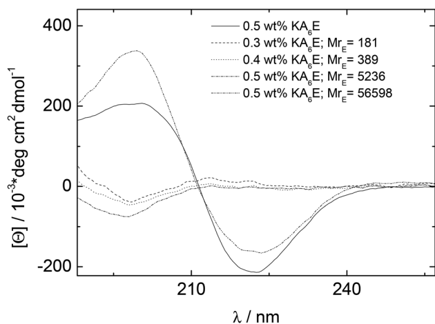
Fig. 4 CD results measured for 0.5 wt% \text{KA}_6\text{E} Trizma pH 8, and samples containing (0.30–0.5) wt% \text{KA}_6\text{E} with \text{Mr}_E \sim (180\text{--}5700) .
