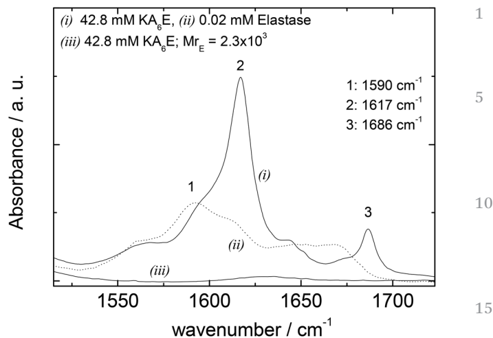
Fig. 5 FTIR data for 42.8 mM \text{KA}_6\text{E} , 0.02 mM elastase and a mixture (42.8 mM \text{KA}_6\text{E} ; \text{Mr}_E = 2.3 \times 10^3 ), in Trizma pH 8.
