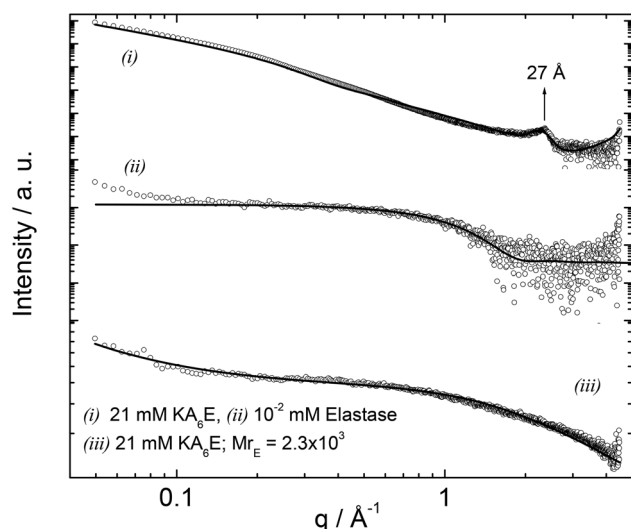
Fig. 8 SAXS curves measured for 21 mM \text{KA}_6\text{E} , \text{Mr}_E = 2.3 \times 10^3 , in Trizma pH 8 and the corresponding controls. The full lines represent the fitting to the data as described in the text.
