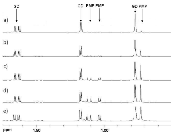
Figure 3 ^1\text{H} NMR stack plot of the breakdown of GD in bis-tris (20 mM) buffered solutions at pH 6.5 in the presence of 100 mol-% of compounds 1 . Time = a) 0 hrs b) 3 hrs c) 7 hrs d) 12 hrs and e) 18 hrs. © Crown Copyright, Dstl.
