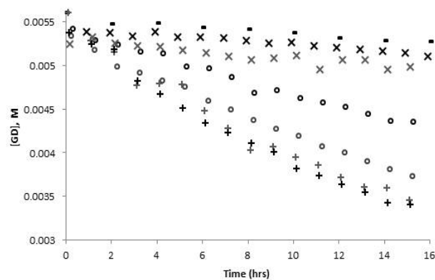
Figure 4 Concentration of GD present as a function of time in bis-tris buffered solutions (20 mM) at pH 6.5 in the absence (-) and presence of 100 (+) and 50 (o) mol-% compound 1 (+) and 100 mol-% compound 3 (x) as determined by ^1\text{H} NMR analysis. © Crown Copyright, Dstl.
