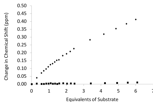
Figure 5 Change in chemical shift of amide NH from compound 3 with the addition of PMP/DMMP (♦/■).
