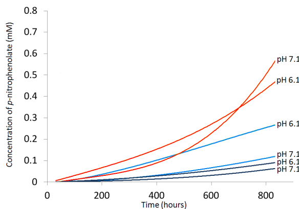
Figure 2 Increasing concentration of p -nitrophenolate formed as BNPP is broken down under different pH conditions with the addition of 100 mol-% compound 2 (—) and 3 (—) with respect to BNPP. The background rate of BNPP breakdown under these conditions was also monitored (—). Data shown is that of the raw data fitted to a curve. Residual R^2 values for the individual fittings \leq 1\% . Blank fitting is taken from an average of two experiments. Individual fitting and calculations can be found in the ESI.
