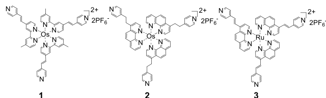
Scheme 1. Chemical structures of the polypyridyl complexes (1-3). 5,7
