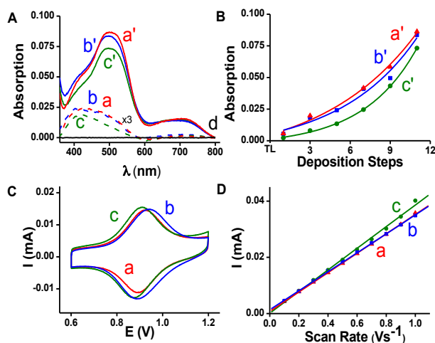
Figure 1. Optical (UV/vis) spectroscopy (A, B) and cyclic voltammetry (CV) (C, D) data. A. Absorption spectra of (a) TL used for the built-up of a 1 -based SPMA, (b) TL generated after disassembly of the 1 -based SPMA with \text{PET}_3 , (c) replicated TL'. (a-c; enlarged 3x for clarity), and (a'-c') are the 1 -based SPMA on ITO-coated glass substrates functionalized with (a') TL formed by reacting a CL with complex 1 , (b') TL after disassembly of the 1 -based SPMA with \text{PET}_3 , (c') replicated TL'. (d) baseline. B. Exponential correlation between the intensities of the MLCT bands ( \lambda \approx 500 \text{ nm} ) and the number of complex 1 deposition steps for the SPMA (a'-c') built on the three TLs (a-c). C. Cyclic voltammograms of TLs (a-c). The scan rate is 400 \text{ mVs}^{-1} . D. Plot of peak currents as a function of the scan rate of the TLs (a-c), with R^2 > 0.98 for the linear fits (see ESI for experimental details).
