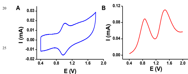
Figure 2. A. Representative cyclic voltammogram (CV) of the replicated 2 -based TL' formed by disassembly of 2 - and 3 -based SPMA with \text{PEt}_3 and selective transfer of osmium complex 2 to ITO substrates functionalized with CLs. The scan rate is 400 mVs -1 . B. Differential pulse voltammogram (DPV) of the reaction solution after the disassembly of 2 - and 3 -based SPMA with \text{PEt}_3 . The following conditions were applied: scan rate: 20 mVs -1 , pulse width: 16 ms, pulse amplitude: 50 mV, and pulse period, 200 ms. For both A and B : electrolyte: 0.1 M TBABF 4 /CH 3 CN was used at room temperature. Pt wire and Ag/AgCl were used as counter and reference electrodes, respectively. The functionalized ITO-coated glass substrates were used as working electrodes.
