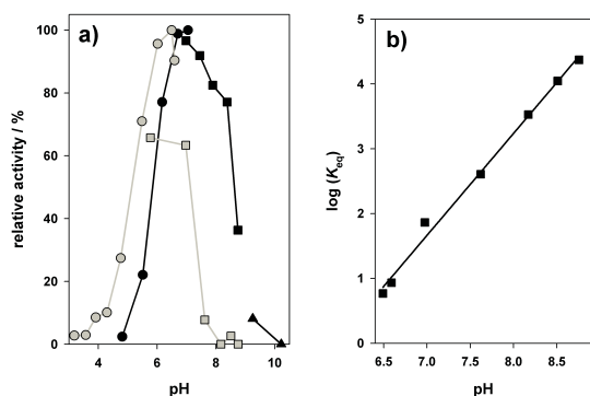
Fig. 1 pH effects on PcOGT activity for phlorizin synthesis and degradation (a), and on the reaction equilibrium constant (b). a) Relative activities of PcOGT ; black symbols (forward reaction: 0.1 mM phloretin, 0.6 mM UDP-glucose, 100% = 18.3 U mg -1 ); grey symbols (reverse reaction: 1.0 mM phlorizin, 2.0 mM UDP, 100% = 5.6 U mg -1 ). The buffers used were citrate (circles), Tris (squares), and CAPS (triangles). b) K_{eq} is for synthesis of phlorizin and UDP from phloretin and UDP-glucose.
