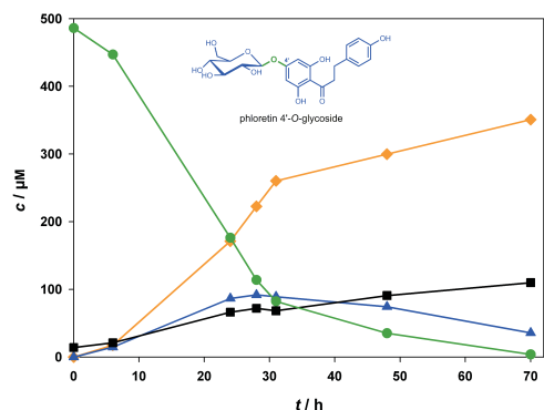
Fig. 3 Conversion of 0.5 mM phlorizin (green) by I121D mutant of OsCGT ( 2.5 \mu\text{M mL}^{-1} ) in the presence of 5 mM UDP and 1 mM UDP-glucose. Further symbols: phloretin (black), nothofagin (orange), 4'- O -glucoside of phloretin (blue).
