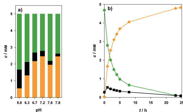
Fig. 2 Conversion of phlorizin (5 mM) via O - to C -glycosidic bond rearrangement in the presence of 2 mM UDP using 100 mU mL -1 PcOGT and 50 mU mL -1 OsCGT . a) Product distribution after reaction for 5 h at different pH conditions. b) Reaction time course at pH 7.0. Colours show phlorizin (green), nothofagin (orange), and phloretin (black).
