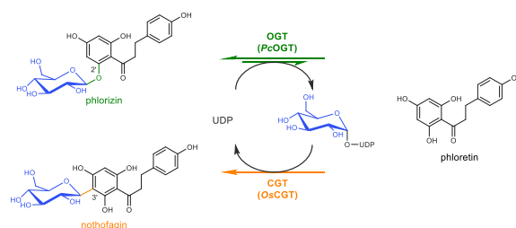
Scheme 1 Conversion of phlorizin into nothofagin, using direct O - to C -glucoside rearrangement in two catalytic steps
