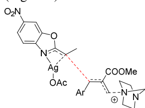
Figure 3: Proposed Transition State
