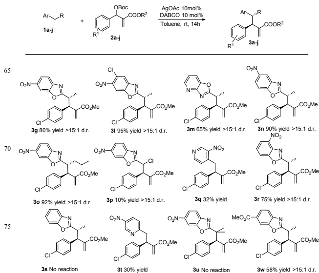
Scheme 3: Reaction scope using alkyl azaarenes 12
