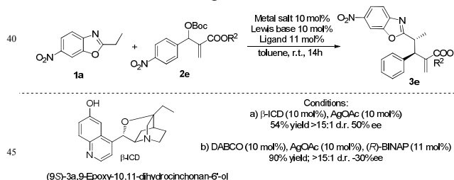
Scheme 4: Asymmetric addition of benzoxazole 1a to MBH carbonate 2e
