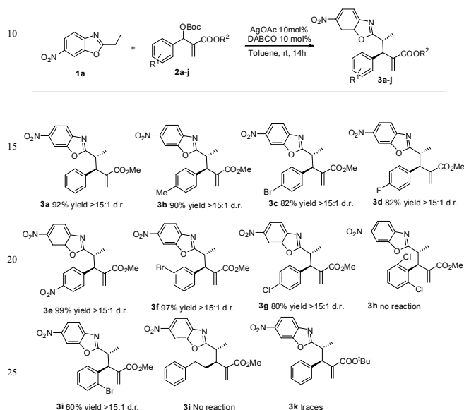
Scheme 2: Reaction scope using MBH carbonate 12
