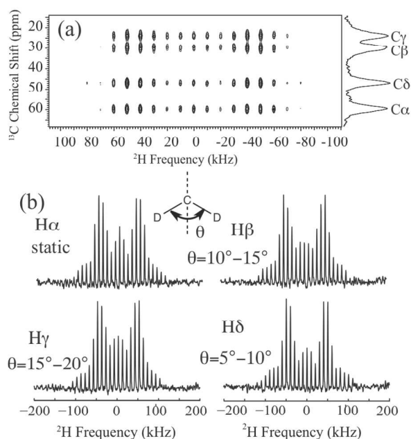
Fig. 2 (a) ^2\text{H} - ^{13}\text{C} HETCOR MAS NMR spectrum for U- [ ^2\text{H} , ^{13}\text{C} , ^{15}\text{N} ] Pro labelled A. aurantia dragline silk. (b) Pro ^2\text{H} line shapes extracted from the 2D spectrum and the proposed dynamics for each site. Pro side-chain dynamics is described by each \text{CD}_2 undergoing fast reorientation between two sites separated by an angle \theta . The angles are extracted from comparing experimental ^2\text{H} line shapes with simulations (see ESI).
