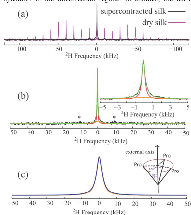
Fig. 3 (a) ^2\text{H} solid-echo MAS NMR spectra for U- [ ^2\text{H} , ^{13}\text{C} , ^{15}\text{N} ] Pro labelled A. aurantia dragline silk in the dry and supercontracted (wet) state. (b) ^2\text{H} solid-echo MAS spectrum of supercontracted (wet) silk (black, same one as show in (a) and its fit (green). The central peak region is expanded and shown on the upper right. A broad (orange) and narrow (red) component was used for the fit. The asterisks indicate the spinning sidebands. (c) Experimental (orange) and simulated ^2\text{H} line shape (blue). The experimental line shape is the broad component extracted from the fit (shown in orange in b). Simulations were performed using SPINEVOLUTION 18 with a model of the entire Pro residue undergoing a three-site reorientation along an external axis with a rate of 3 \times 10^6 \text{ s}^{-1} (the schematic representation of the motion is show on the upper right).
