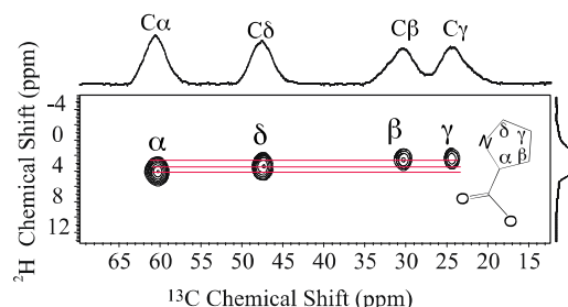
Fig. 1 ^2\text{H} - ^{13}\text{C} HETCOR MAS spectrum for U- ^{2}\text{H}_7 , ^{13}\text{C}_5 , ^{15}\text{N} -Pro labelled A. aurantia dragline silk. Rotor-synchronized sampling in the indirect dimension was used to eliminate spinning sidebands and obtain a narrow spectral-width high-resolution spectrum. The ^2\text{H} - ^{13}\text{C} correlation is indicated for each Pro site in the spectrum (red lines).
