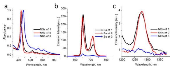
Figure 4. (a) Normalized UV-vis spectra of NSs composed of 1 , 2 and 3 in water. (b) Fluorescence spectra of NSs composed of 1-3 in water (excited at 427 nm; absorbance matched). (c) Emission spectra of singlet oxygen generated by nanospheres containing 1-3 in D 2 O in air saturated solution (excited at 419 nm; absorbance matched).
