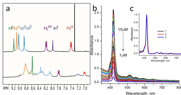
Figure 2. (a) Downfield region 1 H-NMR spectra of (top) porphyrin 1' in CDCl 3 , and (bottom) porphyrin 1 in D 2 O (0.1 M phosphate buffer at pH = 7.0). (b) UV-vis spectra of porphyrins 1 at varying concentrations in H 2 O. (c) Normalized UV-vis spectra of porphyrins 1-3 in THF ( \lambda_{\max} = 421 nm).
