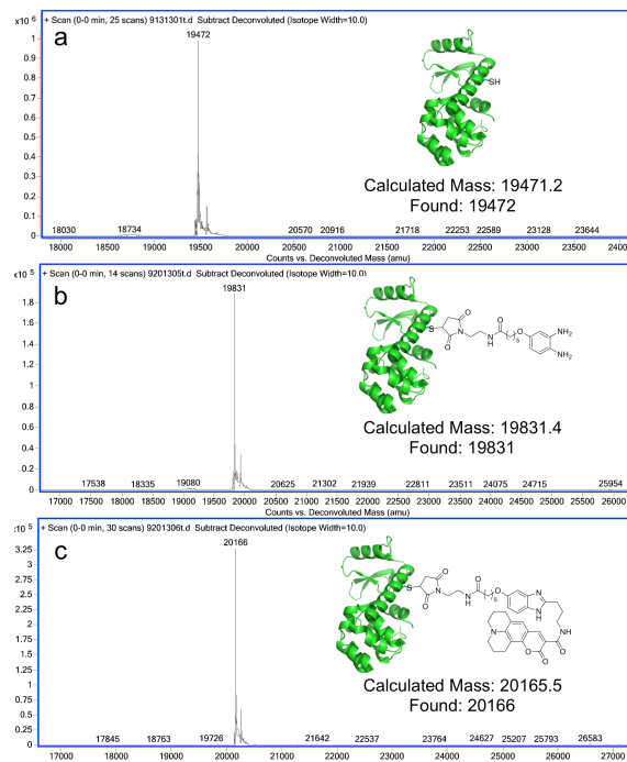
Figure 2. Direct infusion ESI-TOF MS characterization of T4 lysozyme proteins ( a ): T4L-N68C; b ): T4L containing an installed aryl diamine functional group; c ): T4L labeled with an aldehyde Coumarin 343 dye in the presence of 2.5 \mu\text{M} \text{CuSO}_4 ).
