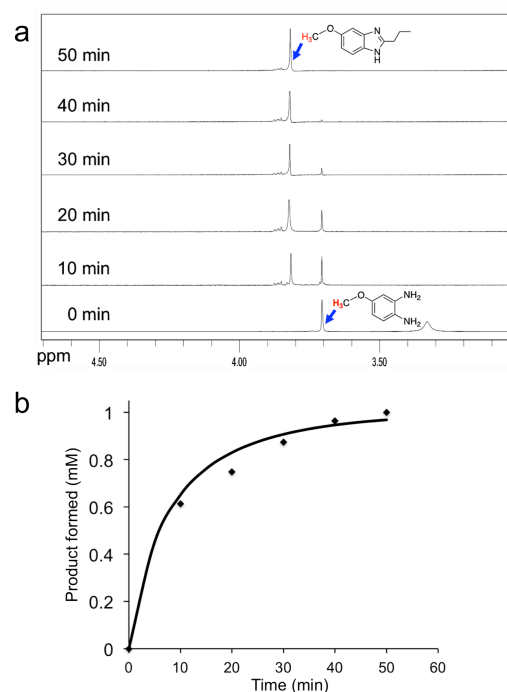
Figure 1. (a) 1 H NMR time course showing the conversion of 4-methoxybenzene-1,2-diamine to its corresponding benzimidazole. (b) Reaction kinetics of the formation of the benzimidazole product over time.
